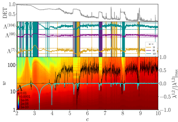
Fig. 6 DET, single scale-specific lacunarities \Lambda(w) and RL curves for varying c \in [2, 10] with n = 2000 for the Roessler system. 95% – confidence bounds are obtained via bootstrapping and excursions outside the indicated horizontals are indicated. Each time series has T = 1000 values after discarding transients. In the lower panel, w –axis and color coding are scaled logarithmically. Black (cyan) curves display the first (second) Lyapunov exponent normalized to their maximum absolute values for better visibility
