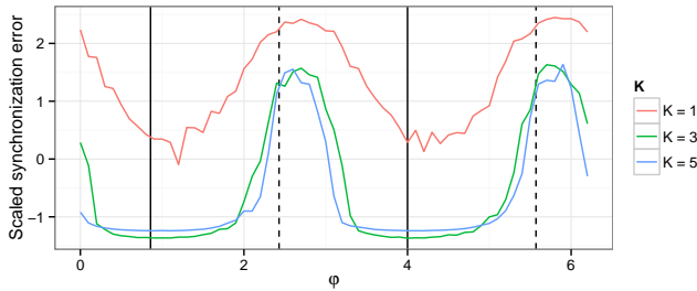
Fig. 3. Cross-section of \varphi versus the scaled synchronization error for several K values at \theta equal to 1.5. The solid vertical lines show the position of the first EOF axis, the dashed vertical line that of the third EOF axis.
