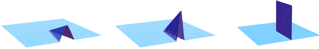
Figure 1: Illustration of \text{gr}F_\nu for \nu = 5 (left) and \nu = 10 (center) and of \text{gr}F (right)
