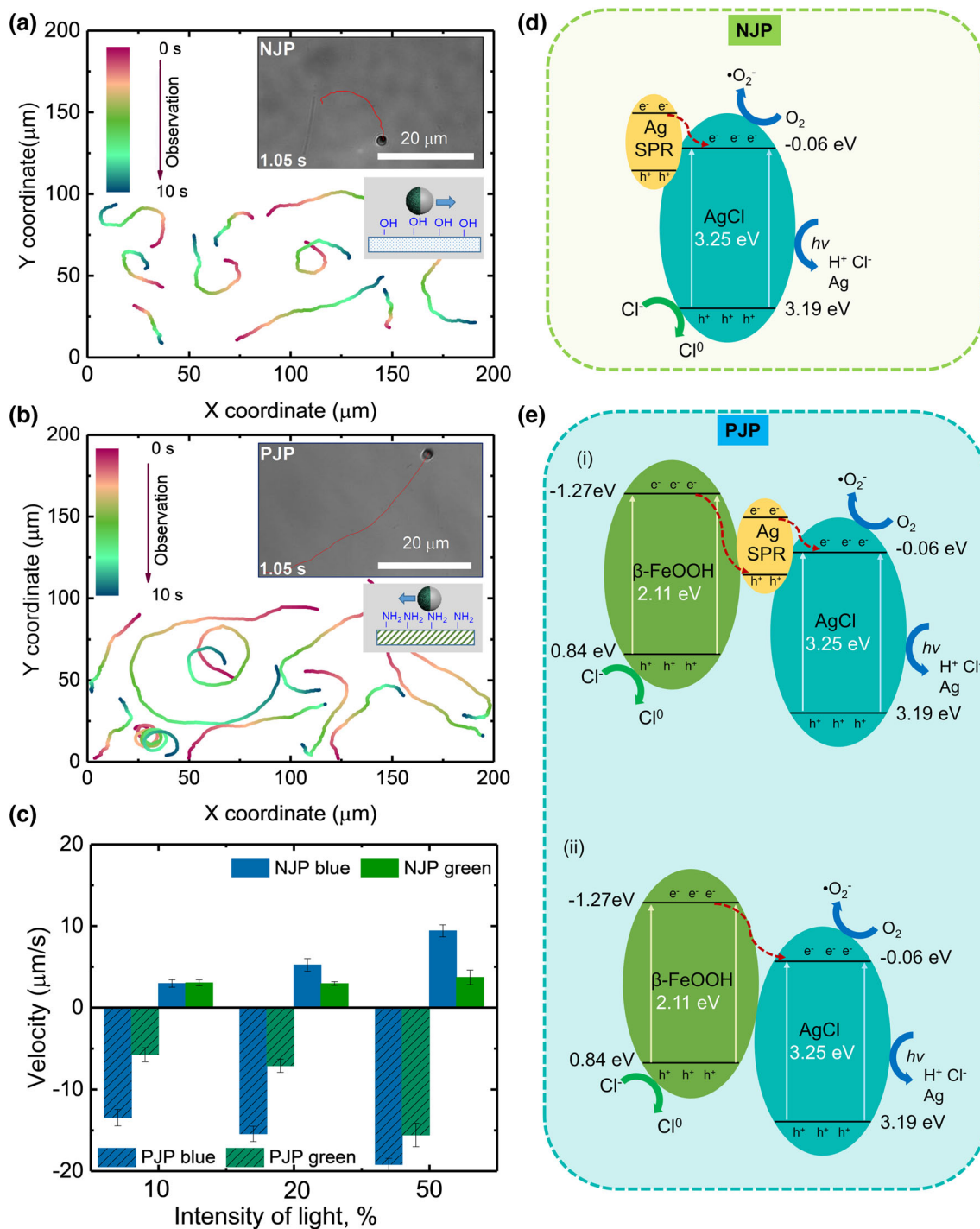
Fig. 2 a Trajectories of Ag/AgCl/PS (NJP) b Trajectories of Ag/AgCl/β-FeOOH/PS (PJP) under blue light illumination for 10 s. c Velocity of Ag/AgCl/β-FeOOH/PS (PJP) and Ag/AgCl/PS (NJP) motors under blue- and green-light illumination with different light intensities. d
