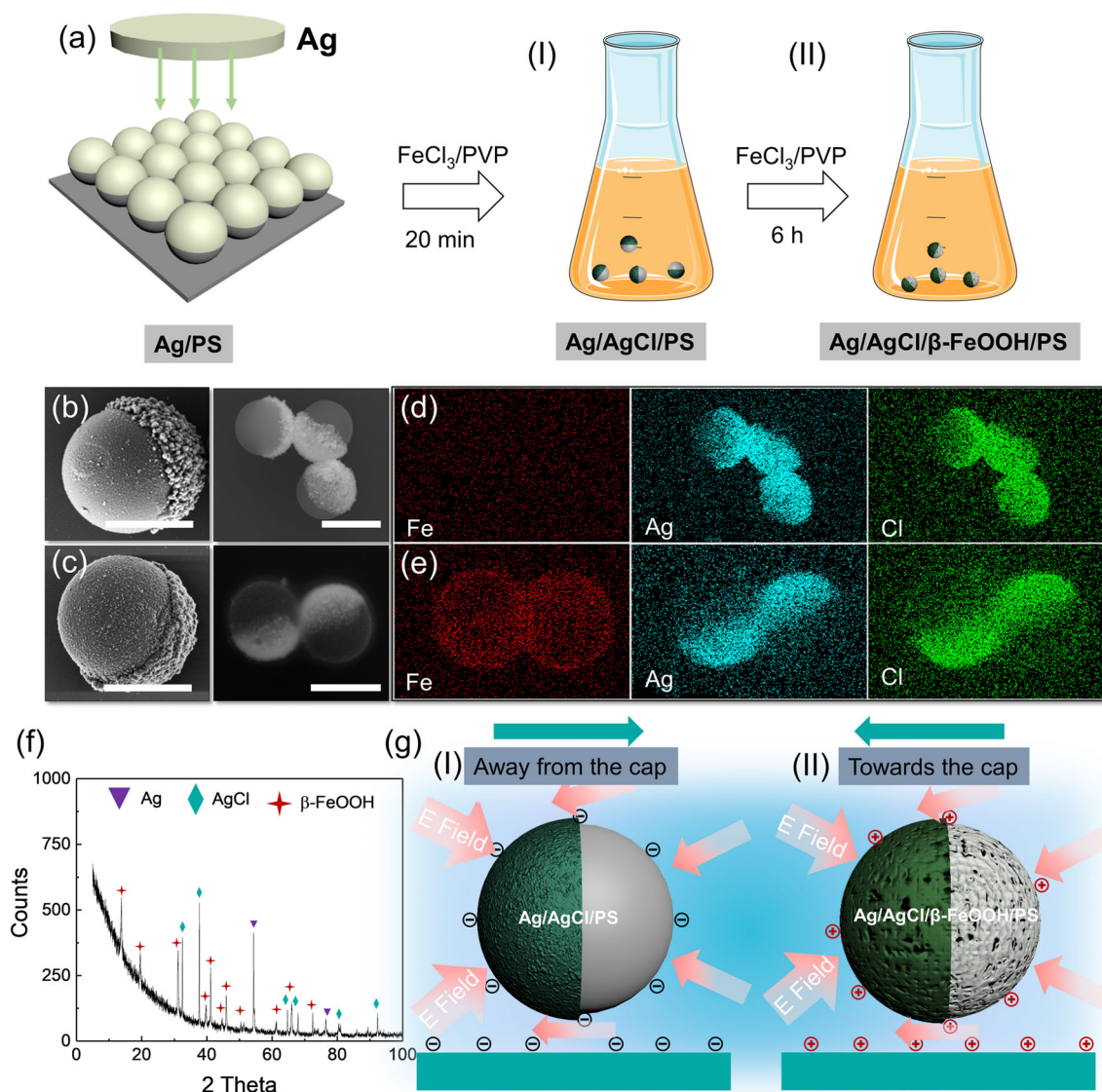
Fig. 1 a Fabrication process of Ag/AgCl/PS (NJP) and Ag/AgCl/ \beta -FeOOH/PS (PJP) micromotors ( b–c ) Scanning electron microscopy (SEM) images of b Ag/AgCl/PS and c Ag/AgCl/ \beta -FeOOH/PS Janus particles. d, e The corresponding EDX mapping of Fe, Ag and Cl elements. f XRD pattern of Ag/AgCl/ \beta -FeOOH/PS Janus micromotor. The peaks indicated by a red star were identified as \beta -FeOOH, International Centre for Diffraction Data (ICDD)
