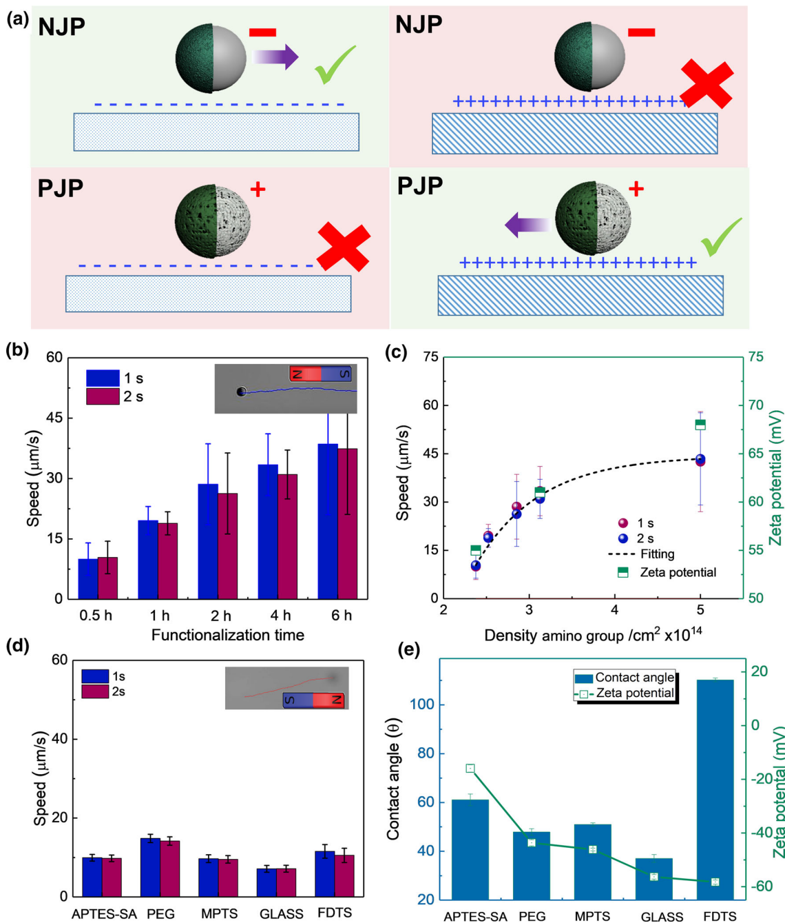
Fig. 3 a PJP and NJP on positively and negatively charged substrate, respectively. b The average speeds of PJP micromotors on positively charged APTES substrates. Error bars are the standard error from ten particles. Insert, the trajectory of magnetic PJP micromotor under a fixed magnetic field. c PJP micromotor speeds and substrate zeta potential change as a function of amino group on the sub-
