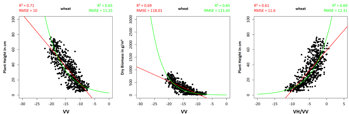
Figure 16. Scatter plots of plant height related to VV backscatter (left) and VH/VV ratio (right) and dry biomass related to VV backscatter (center) for BBCH stages 21–49. Regression lines, R^2 and RMSE are shown in red (linear) and green (exponential).
