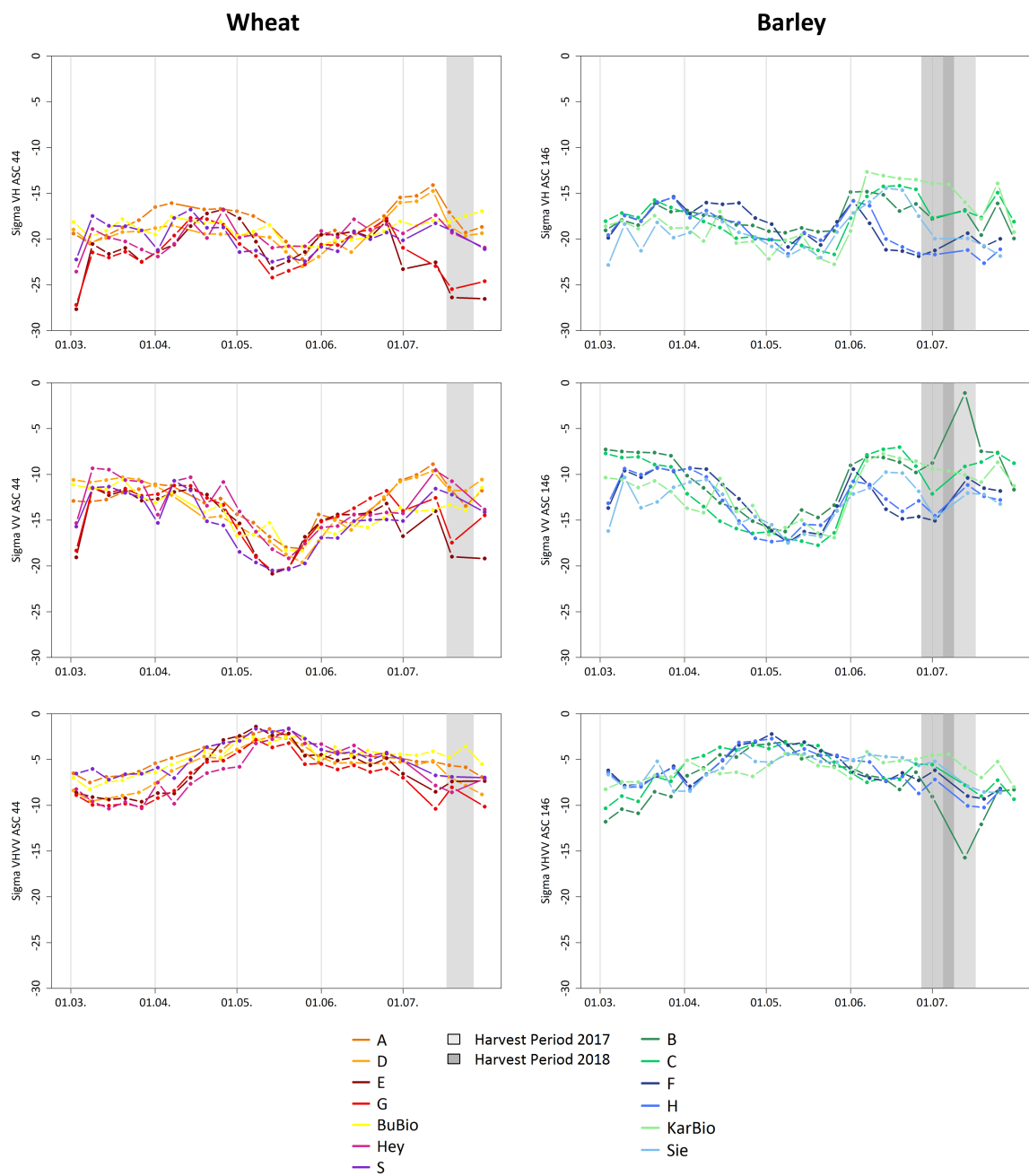
Figure 8. Temporal profiles of backscatter parameters VV, VH and VH/VV of all observed wheat fields (left) and barley fields (right).
