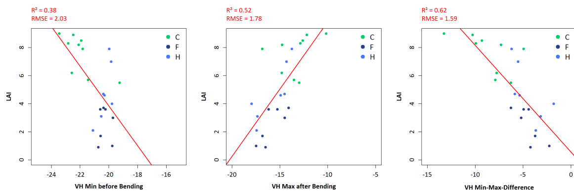
Figure 14. Scatter plots of LAI of three barley fields related to minimum VH backscatter before bending of the ears ( left ), maximum VH backscatter after bending of the ears ( center ) and the difference between both ( right ).
