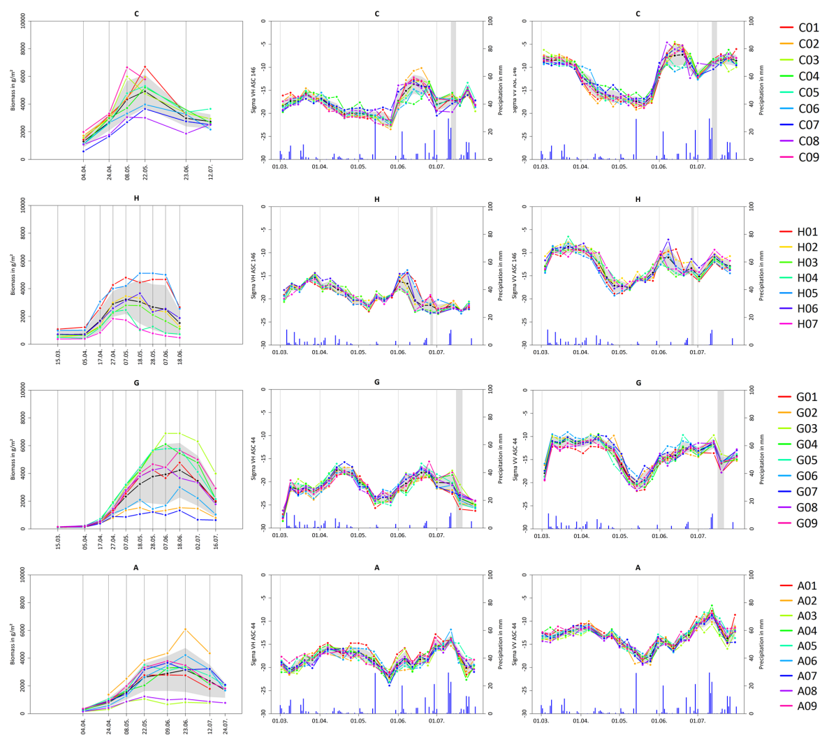
Figure 13. Temporal profiles of single fields: wet biomass (left), VH backscatter (center) and VV backscatter (right). The black line framed by a gray polygon represents the mean value of the field \pm one standard deviation. Gray bars indicate harvest periods, blue bars represent precipitation.
