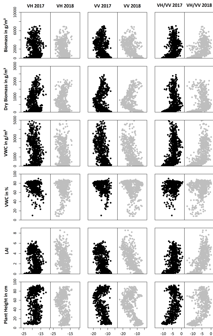
Figure 15. Scatter plots of crop parameters related to backscatter parameters for all wheat fields in 2017 (black points) and 2018 (gray points).
