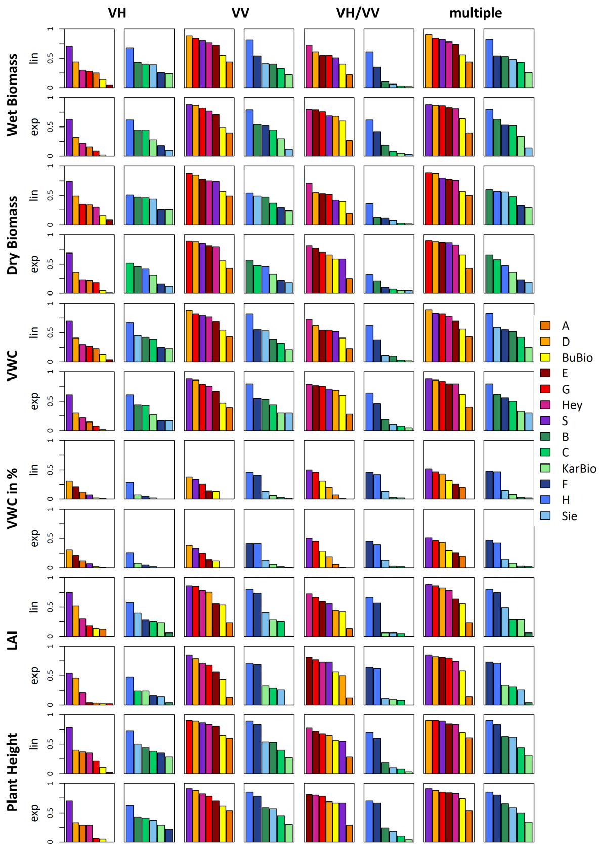
Figure 17. Bar plots of R^2 values of regression between crop and backscatter parameters per crop type for single fields in BBCH stages 21–49.
