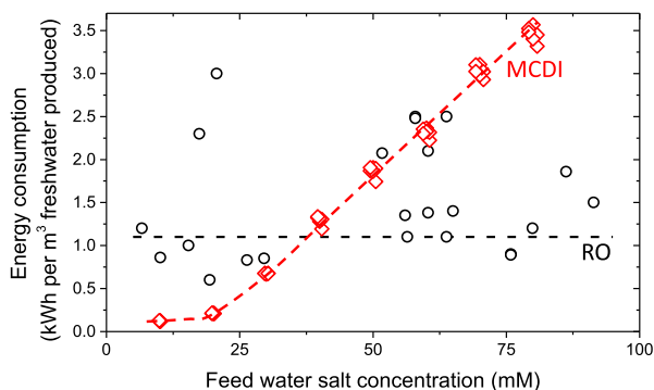
Fig. 19. Energy consumption of water desalination by MCDI and reverse osmosis (RO). Lines serve to guide the eye.
