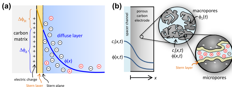
Fig. 10. Models for charge and ion storage in porous CDI electrodes. (a) Structure of the electrical double layer (EDL) according to the Gouy–Chapman–Stern theory for a single planar EDL. (b) Two-porosity-model for the electrode [12,14,23,58]. Both macro- and micropores are electrolyte-filled, and in both we assume locally averaged ion concentrations (within the micropores described by the Donnan model). The large and continuous interparticle pores (macropores) transport salt across the electrode thickness and are charge neutral, with salt concentration c , while in the (intraparticle) micropores the excess ionic charge is charge-compensated by electrical charge located in the carbon matrix.
