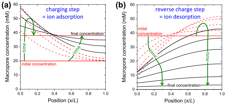
Fig. 14. Calculation results of 1D dynamic porous electrode model for MCDI with a cation exchange membrane located at x = 0 perfectly blocking for anions. (a) Macropore salt concentration profiles as function of time (direction of arrows) during application of -770 mV voltage to the electrode relative to the spacer channel, and (b) After subsequent increase of the potential to +770 mV.
