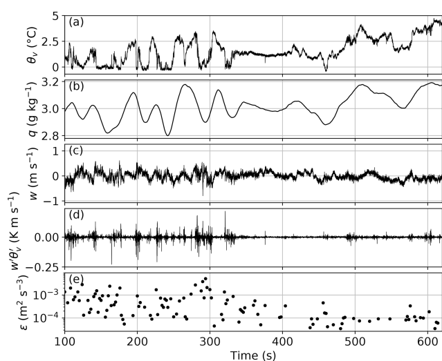
Figure 9. Constant-altitude time series of (a) virtual potential temperature \theta_v , (b) specific humidity q , (c) vertical wind w , (d) covariance \theta_v'w' , and (e) dissipation rate \varepsilon for 6 June measured at 300 m altitude around z_i .
