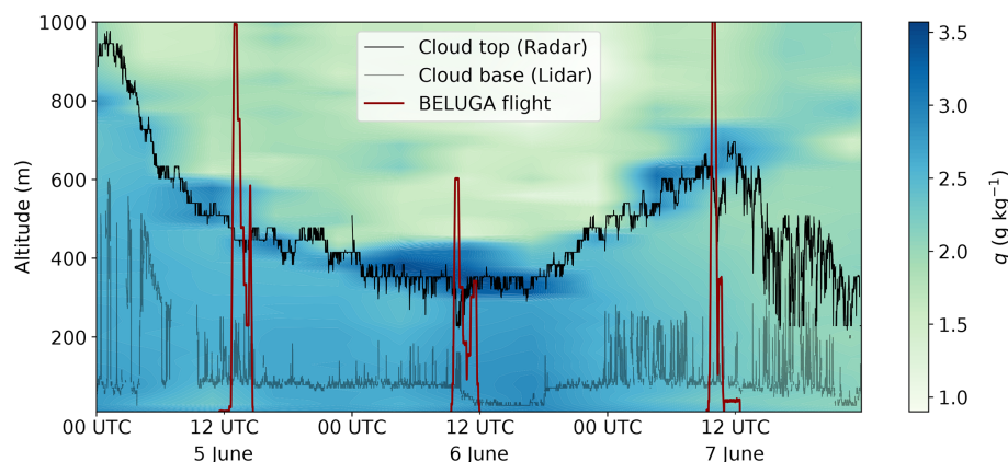
Figure 1. Temporal development of the specific humidity vertical profile observed by radiosondes. The radar-retrieved cloud top height is depicted as a black line; the cloud base height derived from the lidar near-field channel is indicated as a grey line. The red lines represent the BELUGA flight profiles.
