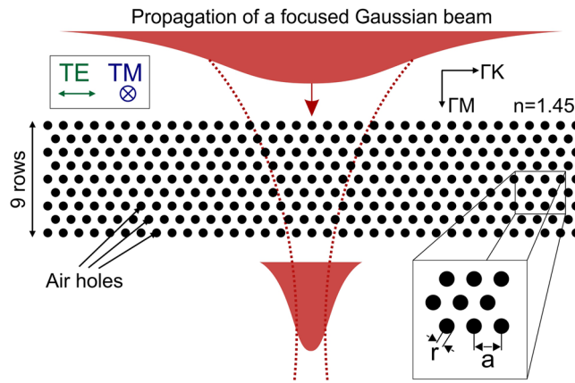
Figure 3. Modeling propagation of the focused Gaussian beam through a triangular lattice photonic crystal to identify transparent configurations. We consider a triangular lattice with 9 rows of air holes in a background with refractive index n = 1.45 . Transparent photonic crystals with isotropic characteristics will allow efficient focusing through the photonic crystal. To model the dependence of the focusing efficiency on the lattice parameters, we start from a Gaussian beam that is focused with a lens with NA = 0.65 through the photonic crystal slab. The insets show the directions of the electric field oscillation for TE and TM polarized light, the \Gamma M and \Gamma K directions of the triangular lattice and the definition of the air hole radius ' r ' and lattice pitch ' a '.
