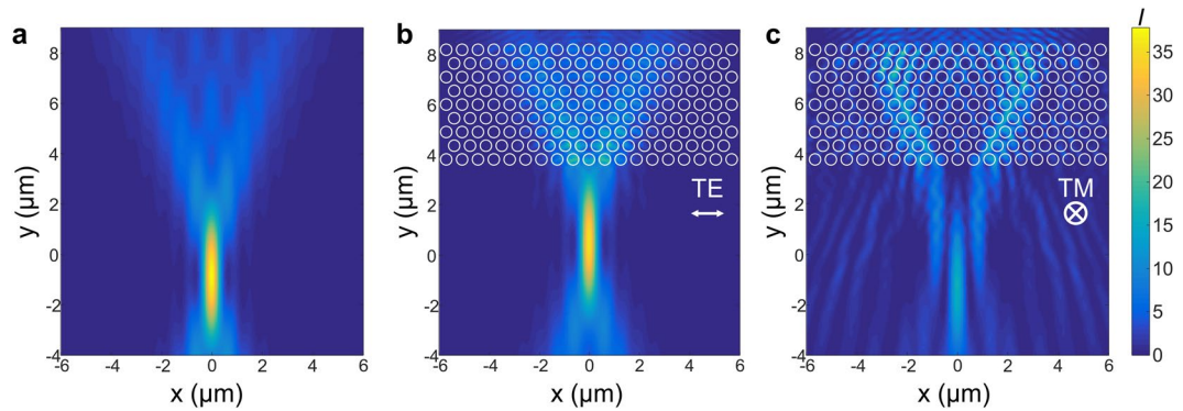
Figure 5. Tight focusing of a beam with \text{NA} = 0.65 lens in case of absence and presence of the photonic crystal for a normalized frequency of 0.8 to demonstrate anomalous transparency. Intensity distribution in the focal region in a dielectric with n = 1.45 when (a) no air holes are present. (b) When 9 rows of air holes are placed on the way of the focused beam for TE polarized light. Efficient focusing takes place owing to anomalous transparency of the photonic crystal at that normalized frequency. (c) The same as b. but now for the TM polarization. The focused beam is scattered due to the non-isotropic behavior of the photonic crystal.
