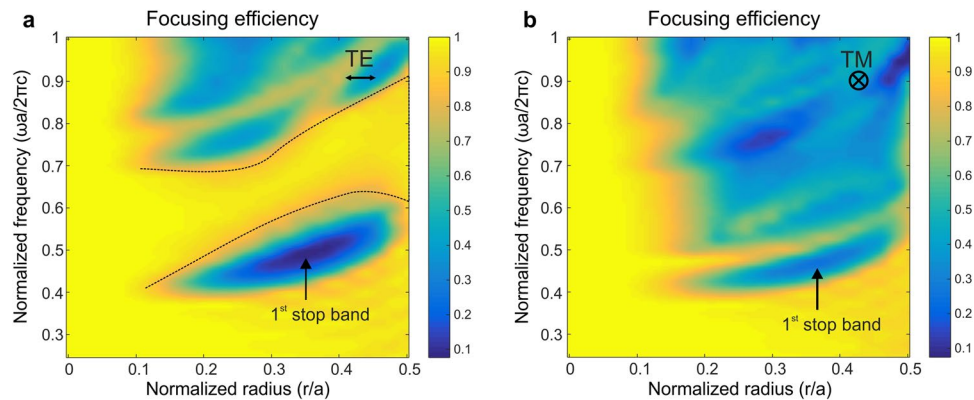
Figure 4. Parameterized study of tight focusing efficiency through a triangular lattice of air holes in a background with refractive index n = 1.45 . The focusing efficiency is calculated as a function of the normalized radius and frequency for TE (a) and TM (b) polarized light, focused through a PhC with 9 rows of air holes along the \Gamma M direction of the lattice (shown in Fig. 3). A region of interest for TE polarization (a) with a high focusing efficiency corresponding to anomalous transparency region of the PhC is marked between 2 dotted lines. For TM polarized light, no such region is observed.
