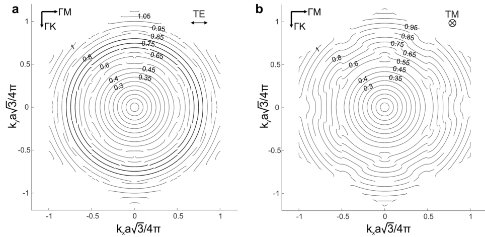
Figure 2. Isofrequency curves for the triangular lattice of air holes. Dispersive characteristics of the photonic crystal with r/a = 0.42 in a background with refractive index n = 1.45 for TE (a) and TM (b) polarizations. In the first figure the isotropic isofrequency curves at high frequencies above the first directional stop band are emphasized with a thicker line.
