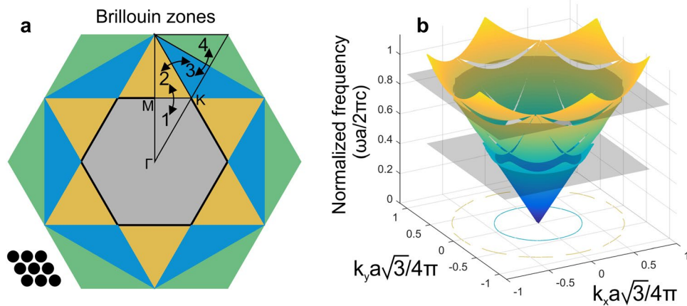
Figure 1. Unfolding procedure of Brillouin zones for a triangular lattice of air holes and photonic band diagram. (a) Illustration of the first four Brillouin zones and their unfolding procedure from the first irreducible zone for a triangular lattice shown in the inset. (b) Photonic band diagram of the two dimensional triangular lattice of air holes with r/a = 0.42 in a background with refractive index n = 1.45 for TE polarization.
