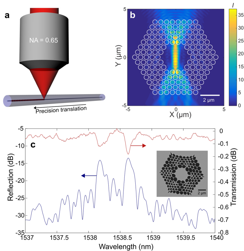
Figure 6. Point-by-point grating inscription in triangular lattice PCF with 5 rings of air holes in the cladding. (a) Outline of the point-by-point grating inscription approach using a high NA lens and fiber placed on a translation stage. (b) Design of the PCF and FDTD modeling result of the propagation of the TE polarized focused Gaussian beam, which demonstrates that high intensity regions are present in the core region and hence that the holey cladding has little influence on the focusing. (c) Reflection and transmission spectrum of the first point-by-point grating inscribed in the triangular lattice PCF with two distinct peaks (and valleys) resulting from the fiber birefringence. Scanning electron micrograph of the fabricated PCF in the inset.
