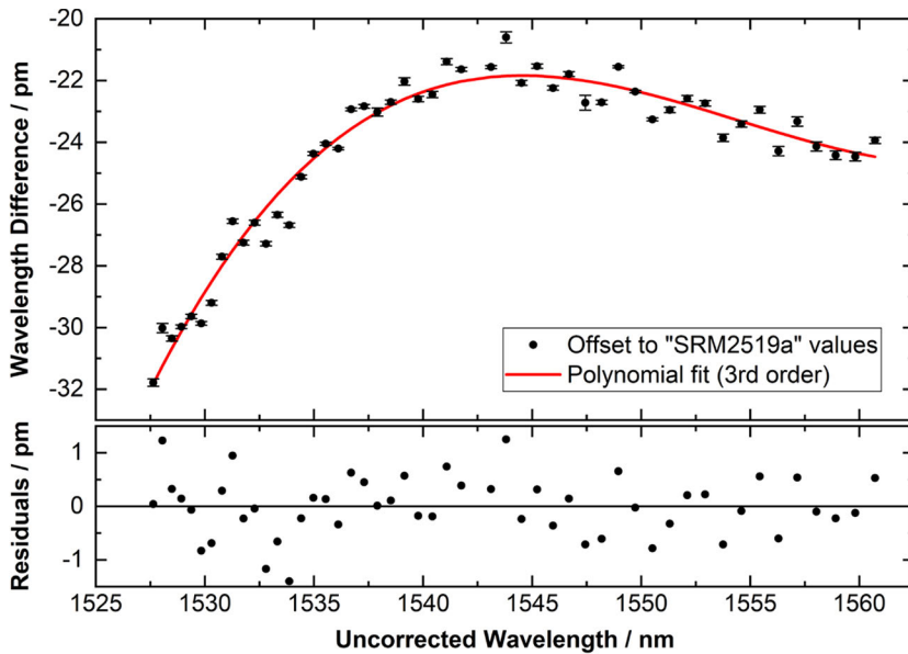
Figure 9: (upper) Difference between the centre wavelength of absorption lines determined by the Voigt fit and the literature values with uncertainty (whisker) from [17]. Polynomial fit (3rd order) used for the wavelength correction of the spectrum (red line). (lower) Residuals of the fit function.
