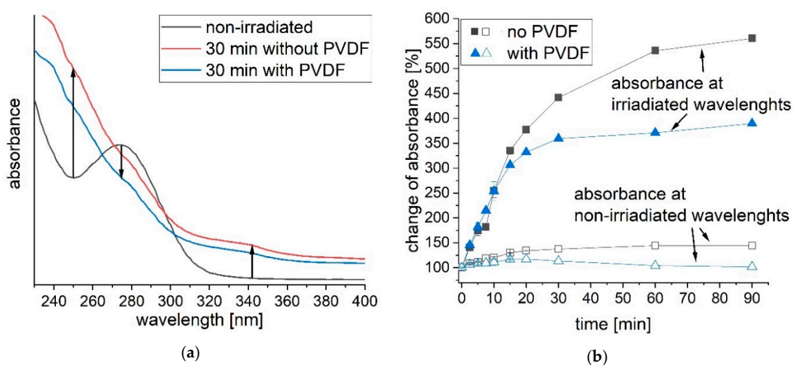
Figure 5. (a) Absorbance spectrum of non-irradiated and 30 min UVA irradiated diclofenac with and without PVDF. (b) The change of absorbance is shown over time for diclofenac UVA irradiation with and without PVDF. The area under the absorbance vs. wavelength was calculated for the non-irradiated region from 230–309 nm and the irradiated region from 309–400 nm. The change of absorbance was calculated by setting the area of absorbance of the non-irradiated diclofenac solution at 100%.
