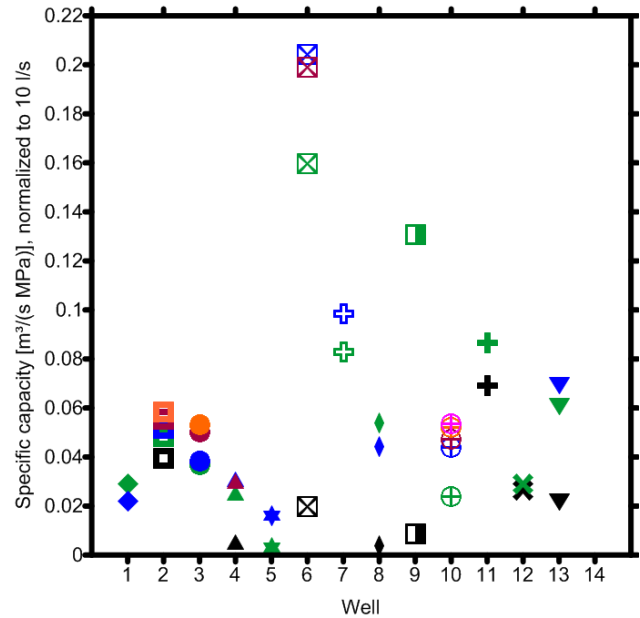
Figure 4. Specific capacity for different wells before and after acidizing (extract of Fig. 3). Colors indicate the time when the pump tests were performed: before first acid treatment (black), after first acid treatment (green), after second acid treatment (blue), after third acid treatment (red), after fourth acid treatment (orange), and after fifth acid treatment (pink).
