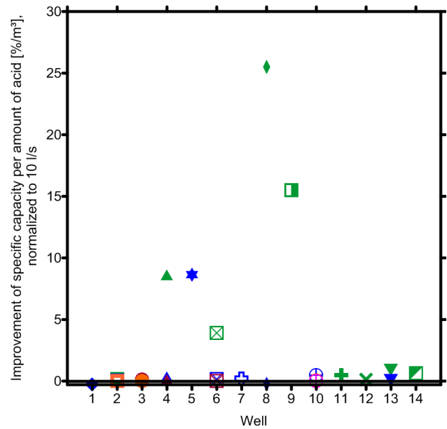
Figure 8. Improvement of the specific capacity normalized to the amount of acid used and a flow rate of 10 L s -1 . Colors indicate the acidizing step that causes the improvement: first (green), second (blue), third (red), fourth (orange), and fifth (pink).
