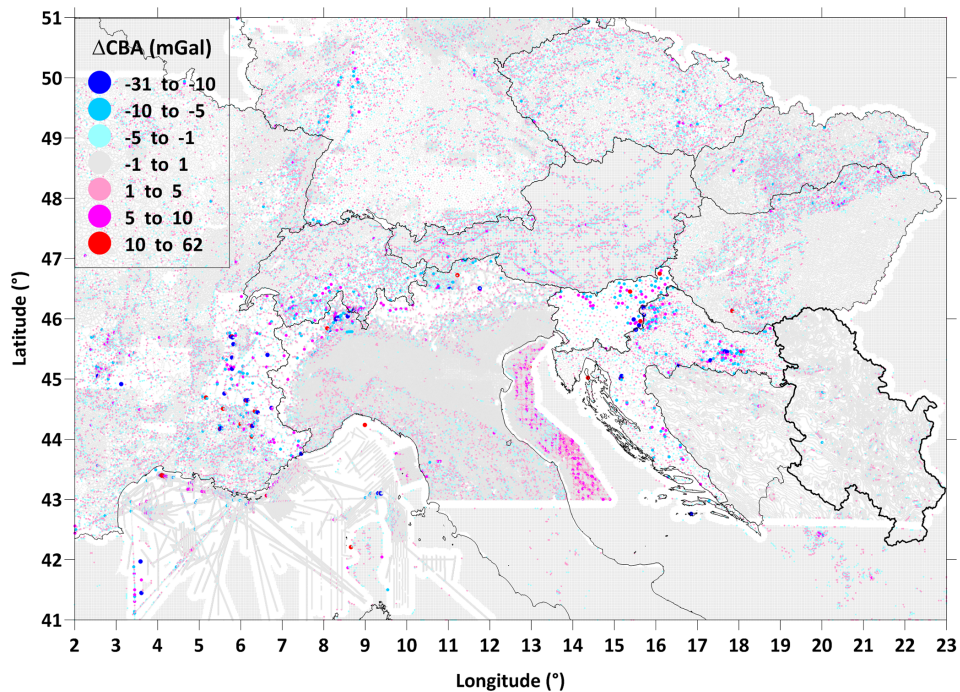
Figure 16. Results of cross validation of the new CBA. The point sizes are proportional to the magnitude of residuals. The grey “background” represents locations with lowest residuals.
