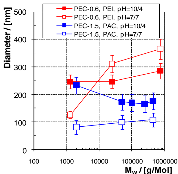
Figure 12. Plot of D_H versus the M_W of PEI or PAC within PEC dispersions of PEI/PAC at c_{PEL} = 0.001 M (all) and n_-/n_+ = 0.6 or 1.5 .
