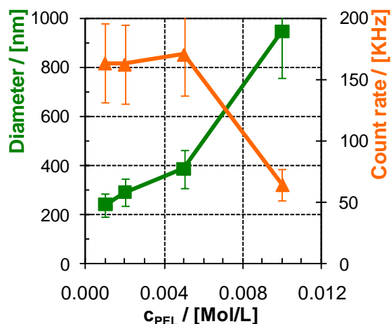
Figure 8. Hydrodynamic diameter D_H and count rate (CR) of PEC-0.6 dispersions of PEI/PAC in dependence of PEL concentration ( c_{PEL} ).
