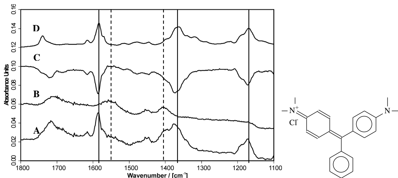
Figure 15. ATR-FTIR spectra of solution casted dry PEC-0.8 films of PEI/PAC ( n_-/n_+ = 0.8 , cationic) (A) loaded with malachite green (MLG); (B) after contact to H 2 O for 15 h; (C) difference (B) minus (A); (D) pure MLG film. IR bands of MLG are labeled by full lines and of PEI/PAC by broken lines. The structure of MLG is given on the right.
