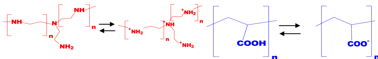
Figure 2. Structural formulae and pH dependence of branched poly(ethyleneimine) (PEI) and linear poly(acrylic acid) (PAC).
