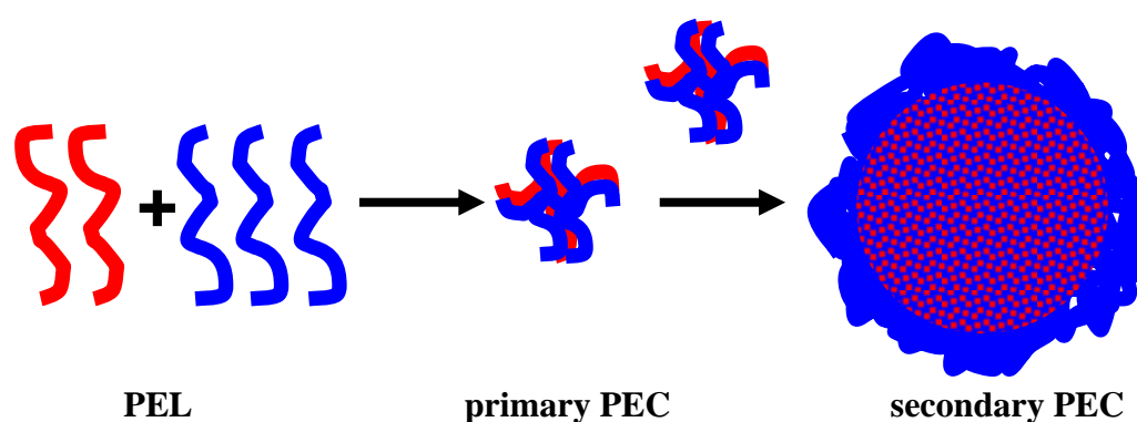
Figure 1. (From [18] with kind permission of Research Trends) Scheme of the polyelectrolyte (PEL) complex (PEC) formation process supported by experiment and simulation [17].
