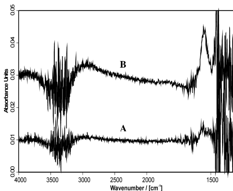
Figure 13. ATR-FTIR spectra of in-situ formed PEI/PAC complexes at n_-/n_+ = 0.5 in contact to cellulose film under the conditions: (A) 1. PEI 2. PAC (0.001 M); (B) 1. PAC 2. PEI (0.001 M) (see text).
