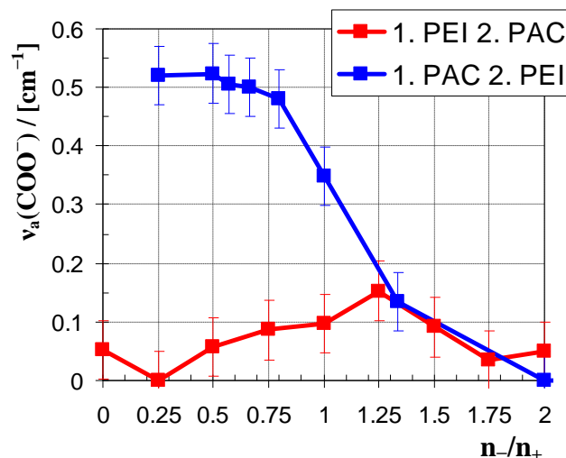
Figure 14. Course of the \nu_a(\text{COO}^-) band integrals diagnostic for the deposition of PEI/PAC complex layers upon dosing either PAC to PEI solution (1. PEI 2. PAC) or PEI to PAC solution (1. PAC 2. PEI) in direct contact with the cellulose model film dependent on mixing ratio n_-/n_+ for c_{\text{PEL}}=0.001 M.
