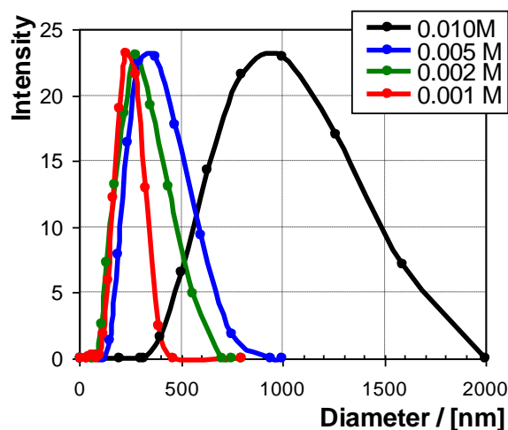
Figure 7. Intensity distributions from DLS data on PEC-0.6 dispersions of PEI/PAC in dependence of PEL concentration ( c_{PEL} ).
