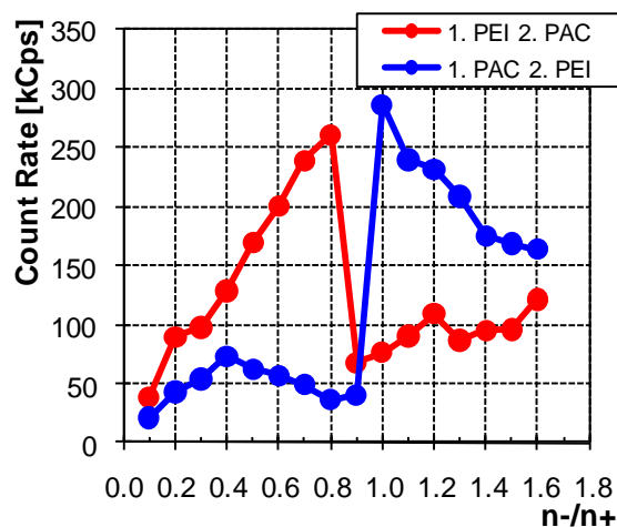
Figure 5. Count rate (CR) of PEI/PAC versus mixing ratio.
