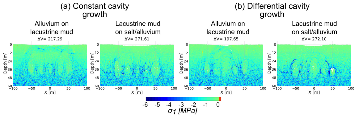
Figure A2. Maximum principal stress around void spaces for (a) constant and (b) differential cavity growth scenarios models. Chosen are two material combinations where the subsrosion-affected layer differs in strength: alluvium-on-mud multilayer and mud-on-salt/alluvium succession. Shown are critical stages after void space installation followed by or exactly during overburden collapse for the same particle assembly. The removed volume [m 3 ] is shown above the plots.
