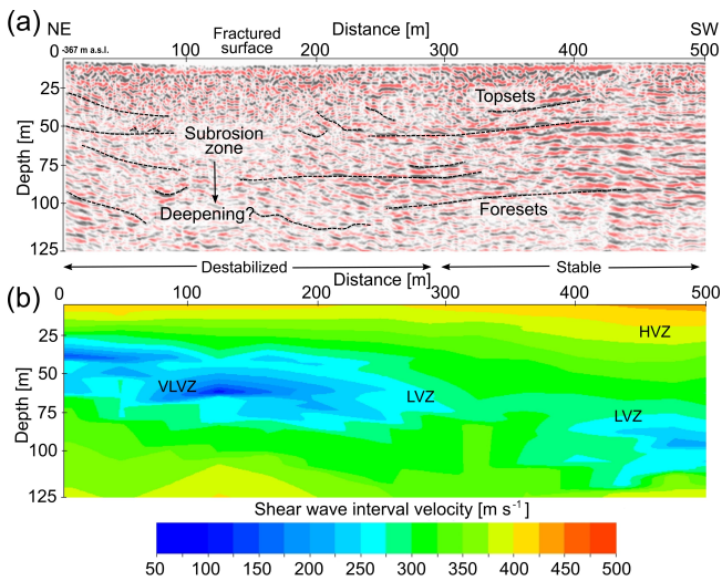
Figure 12. Subrosion-affected parts of shear wave reflection seismic profile 1 at the sinkhole site of Ghor Al-Hadiitha. (a) Modified and interpreted first 500 m of profile 1 after Polom et al. (2018). (b) Shear wave interval velocity versus depth with marked very-low- (VLVZs), low- (LVZs) and high-velocity zones (HVZs).
