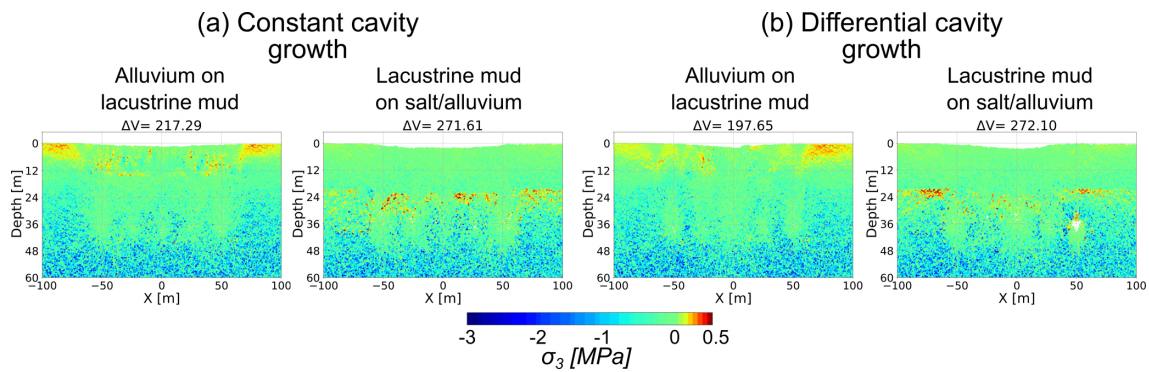
Figure A3. Minimum principal stress around void spaces for (a) constant and (b) differential cavity growth scenarios models. Chosen are two material combinations where the subsrosion-affected layer differs in strength: alluvium-on-mud multilayer and mud-on-salt/alluvium succession. Shown are critical stages after void space installation followed by or exactly during overburden collapse for the same particle assembly. The removed volume [m 3 ] is shown above the plots.
