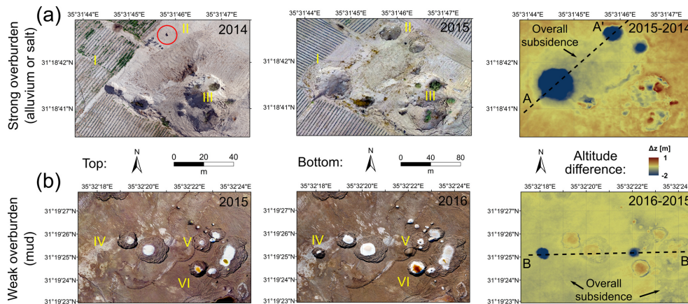
Figure 10. Examples for subsidence and sinkhole formation at Ghor Al-Haditha from orthophotos and DSM difference maps. All orthophotos and DSMs have the same resolution ( 10\text{ cm px}^{-1} ) and the accuracies (horizontal, vertical) are as follows: 2014 (10, 11 cm), 2015 (12, 17 cm) and 2016 (37, 31 cm). (a) Vertical displacement between 2014 and 2015 in the alluvium. Large sinkholes have formed in the alluvium (I, II) with slight overall subsidence along cross-section A–A’ from SW to NE. The red circle marks a small precursory hole at (II). Vegetation growth may cover subsidence effects in coalesced sinkholes (III). (b) Vertical displacement changes between 2015 and 2016 in the mud flat. Precursory information (reactivated sinkholes) may exist (IV) or not be visible (V). Nests of sinkholes exist (VI) in an area of pronounced overall subsidence of 0.5\text{ m} \pm 0.2\text{ m} determined for cross-section B–B’ from W to E. Compare topographic profiles in Fig. 11.
