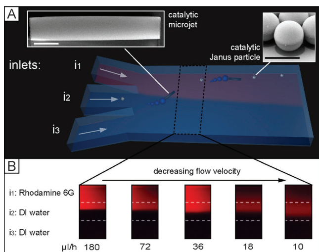
Figure 1. Chemotactic attraction of catalytic micromotors in a microfluidic device. A) Three-dimensional scheme of a microfluidic flow cell with three merging inlets in \Psi -shape ( i_1 , i_2 , and i_3 ) on the left and one larger outlet on the right. Inlet i_1 contains the fuel for catalytic motors, which are introduced through inlet i_2 and depicted in the insets on the top left (microtubes) and top right (Janus particles). i_3 contains water. Scale bar: 5 \mu\text{m} . B) Flow test using fluorescent Rhodamine as model introduced in i_1 to visualize flow-speed-dependent diffusion of the dye molecules across the channel.
