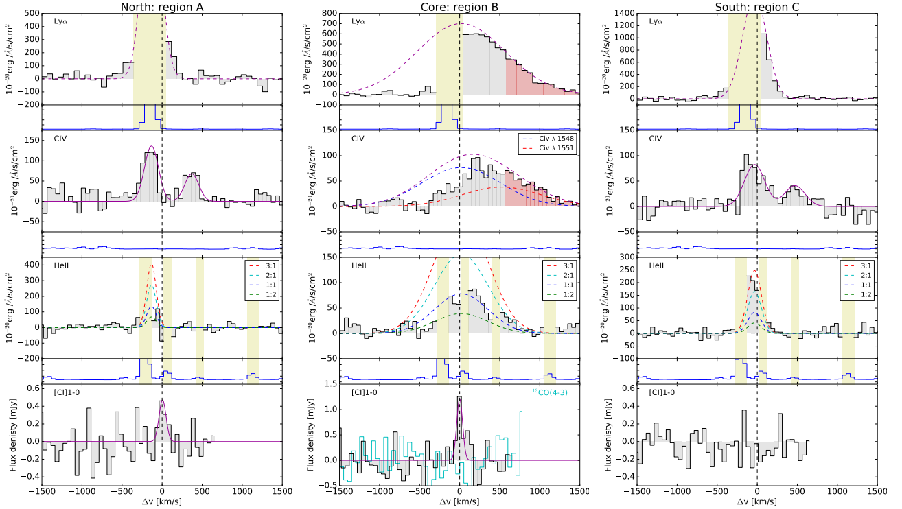
Fig. 4. Extracted spectra of three different regions, as indicated in Fig. 3. Left to right: northern, core, and southern regions of the same emission line (which is indicated in the top left corner of each panel). Top to bottom: Ly \alpha , C IV, and He II from the MUSE cube and [C I] from the ALMA cube for each of the three regions. The abscissa in each panel is the velocity relative to the systemic redshift in units of km s ^{-1} , estimated using the redshift of the [C I] line at the core; the dashed vertical black line indicates the systemic velocity, which is set to zero. The ordinate in each panel is the flux density in units of erg s ^{-1} cm ^{-2} Å ^{-1} . In the panels that show the extracted spectra around the wavelengths of the Ly \alpha , C IV, and He II emission lines, we indicate velocity (wavelength) regions that are strongly affected by night sky lines with yellow shading, and these regions are completely ignored for any fits to the line profiles. The purple lines show the best fitting line profiles, while the dashed lines indicate those fits where a significant part of the line has been ignored in constraining the fit (Sects. 3.1 and 3.2). The red shaded part of the Ly \alpha and C IV spectrum of region B indicates the part that was used for the line fitting, and the dashed blue and red lines indicate the individual part of the C IV doublet. Most of the flux in regions A and C is lost due to the impact of the strong night sky line at 5577 Å. Dashed blue, green, cyan, and red lines indicate possible He II line profiles, assuming that the relative velocity and FWHM are the same as that for the C IV line and have flux ratios He II/C IV of 0.5, 1, 2, and 3. The solid cyan curve in the lowest middle panel indicates the spectrum of the ^{13}\text{CO}(4-3) line around the systemic velocity (it is a non-detection and this is simply a spectrum of the noise).
