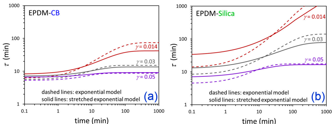
Figure 9. Time-dependent \tau from fictive strain model fits for down-jump experiments from equilibrium at \gamma = 0.25 to the indicated \gamma values for EPDM-CB (a) and EPDM-Silica (b). The dashed lines are from the exponential model and the solid lines are from the stretched exponential model.
