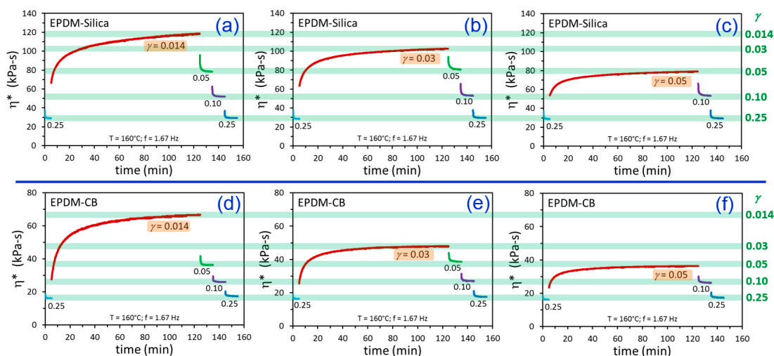
Figure 4. Time-dependent dynamic viscosity results for EPDM-Silica (a–c) and EPDM-CB (d–f) from testing using the indicated strain amplitude histories. The green bars represent the apparent equilibrium \eta^* values at the various values of \gamma . Note the different y-axis scalings for EPDM-Silica (a–c) and EPDM-CB (d–f).
