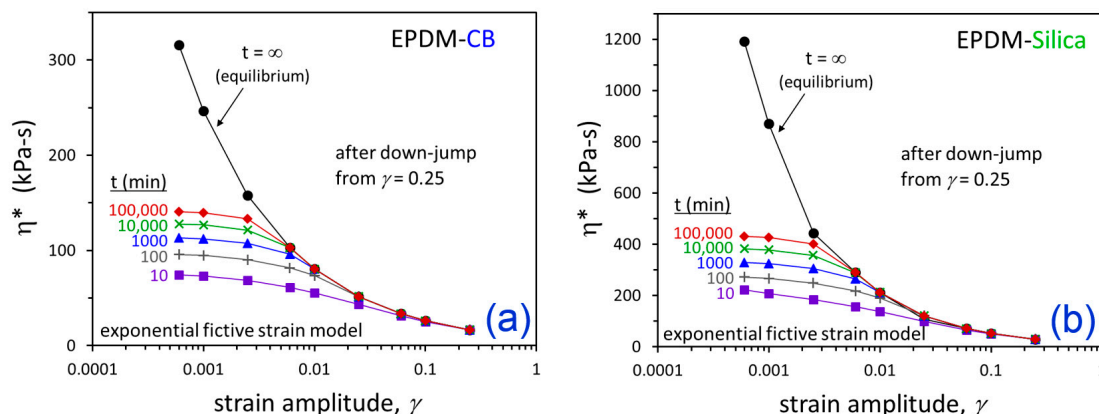
Figure 11. Predicted \eta^* vs. \gamma at the indicated times for EPDM-CB (a) and EPDM-Silica (b) using parameters from fitting the experimental data (Figures 8 and 9). Note the different y-axis scalings for (a,b).
