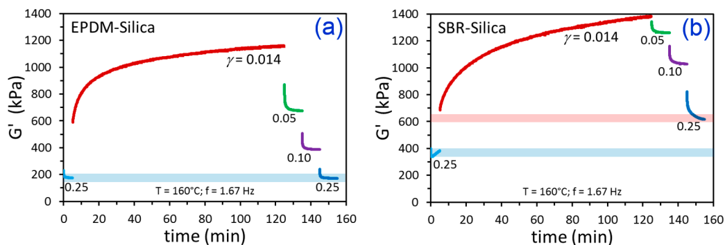
Figure 3. Time-dependent G' results from the indicated strain amplitude history for EPDM-Silica (a) and SBR-Silica (b). The blue bar in (a) represents the similar starting and ending values of G' at \gamma = 0.25 . In (b), the blue bar is the starting G' at \gamma = 0.25 and the pink bar is the final G' at \gamma = 0.25 , which is higher.
