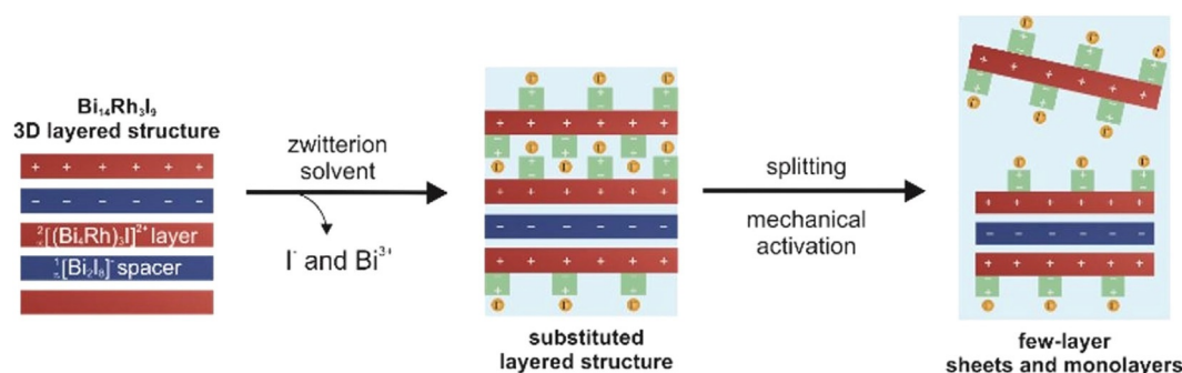
Scheme 2. Scheme of the substitutive approach to exfoliate Bi 14 Rh 3 I 9 . Splitting can be amended by suitable solvents and sonomechanical treatments.
