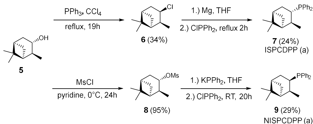
Scheme 1. Synthesis of the ligands isopinocampheyl-diphenylphosphine (ISPCDPP) (7) and neoisopinocampheyl-diphenylphosphine (NISPCDPP) (9). (a) For purification, the ligands were converted to the corresponding borane adduct.
