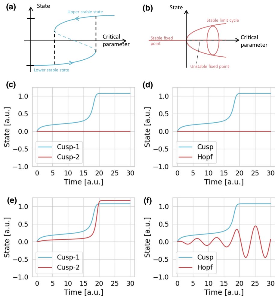
Fig. 2 The bifurcation diagrams of the pre-implemented tipping elements are shown, which possess a Cusp- or a Hopf-bifurcation, respectively ( a and b ). Further, two examples of tipping events are shown, once for the case where no tipping cascade emerges ( c and d ), and once where a tipping cascade emerges ( e and f ). a Bifurcation diagram of a fold-bifurcation (see Eq. 3). b Bifurcation diagram of a (supercritical) Hopf-bifurcation (see Eq. 4). c Two cusp differential equations with the parameters a_1 = a_2 = 4 , b_1 = b_2 = 1 , x_{0,1} = x_{0,2} = 0.5 and c_1 = 0.2 , c_2 = 0 . Thus, the first tipping element is slightly pushed over its
