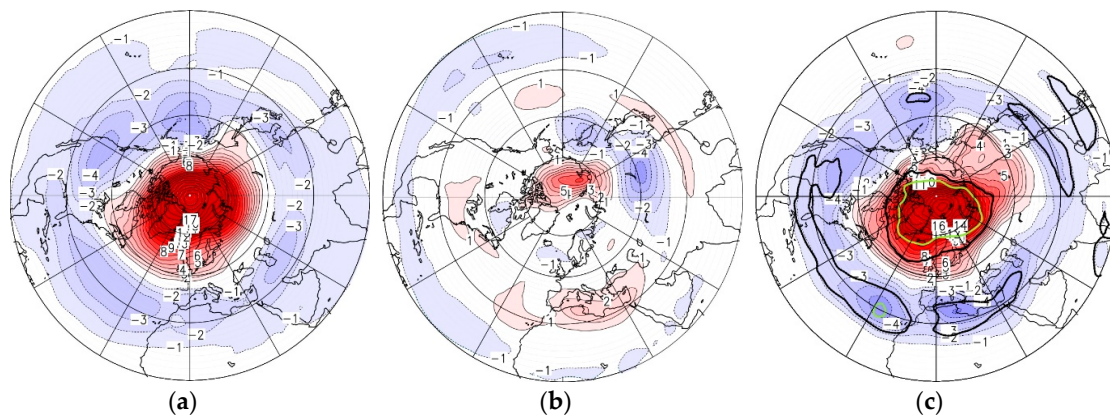
Figure 6. Stereographic maps of mean total ozone (TO3) anomaly ( 10^{-4} kg/m 2 ) for strong-PJO events (a), non-PJO events (b), and difference of strong-PJO minus non-PJO events (c) for ERA-Interim averaged over 15 days after CD. Thick black (green) line in (c) includes significant areas with differences of 80% (95%) confidence. Total ozone means column integrated ozone.
