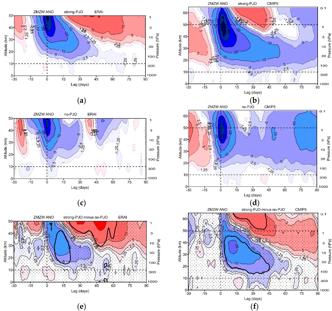
Figure 2. Same as Figure 1 but for the evolution of zonal mean zonal wind (ZMW) anomaly (m/s) averaged between 50° and 70° N.
