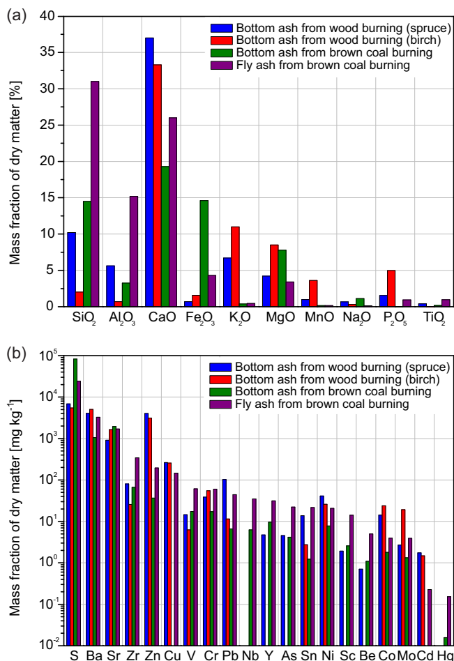
Figure 2. Mass fractions of (a) certain oxides and (b) additional elements in the dry matter of bottom ash from spruce, birch, and brown coal burning, as well as fly ash from brown coal burning. The analysis was performed by means of inductively coupled plasma-sector field mass spectrometry (ICP-SFMS) at ALS Scandinavia AB (Luleå, Sweden). Table 3 shows the values given in the bar chart and the associated uncertainties.
