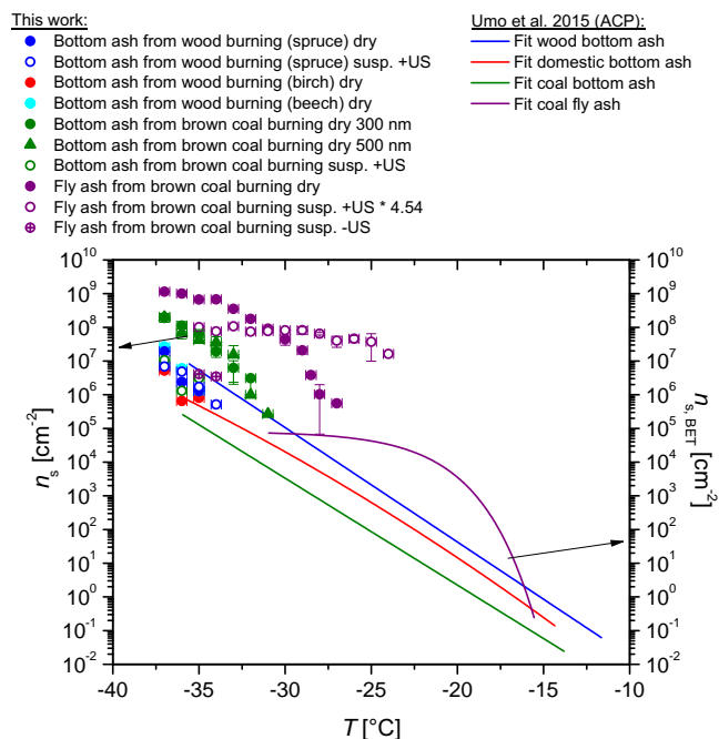
Figure 5. Comparison of ice nucleation surface site density n_s as a function of temperature T for ash particles from dry (full circles: 300 nm particles, triangles: 500 nm particles) and wet generation (open circles: 300 nm particles) with results by Umo et al. (2015, lines). For the LACIS measurements, the particle surface area was determined assuming spherical particles (left ordinate), whereas the n_s values reported by Umo et al. (2015) are based on the BET specific surface area of the particles (right ordinate).
