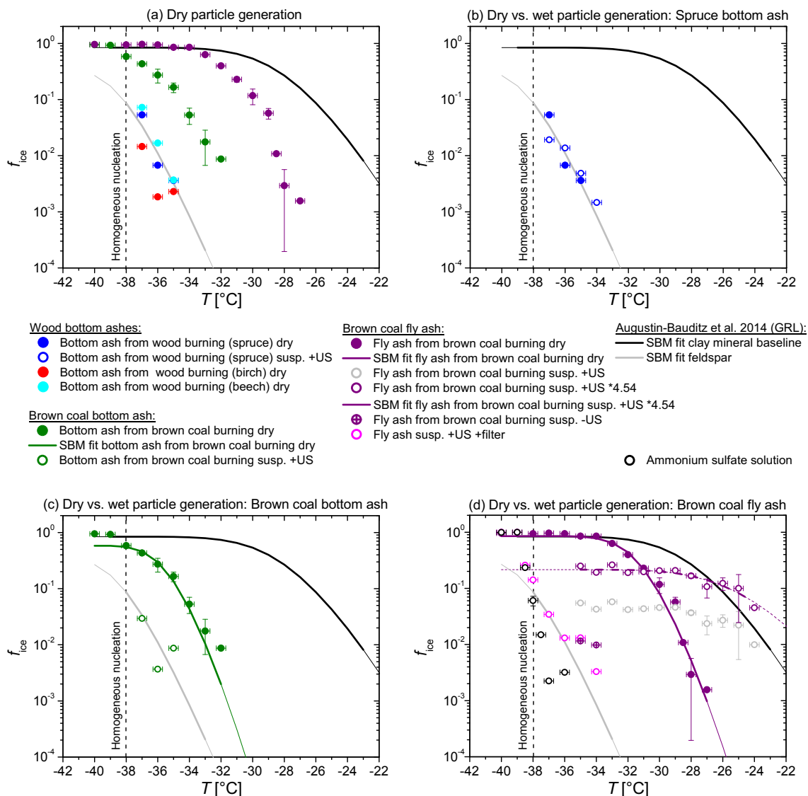
Figure 4. Ice fraction f_{ice} as a function of temperature T for ash particles from dry (full circles) and wet generation (open circles, b , c , d ) with D_{p,el} = 300 nm. Error bars represent the LACIS temperature error of 0.3 K and the f_{ice} standard deviation of three or more measurements, respectively. A scaling factor of 4.54 was applied to the fly ash suspension measurements to account for the occurrence of crystals during wet particle generation. The solid and dashed lines represent the SBM fits to selected samples from this work and to data published in Augustin-Bauditz et al. (2014), all for D_{p,el} = 300 nm. Parameters for the SBM fits are given in Table 4. The feldspar sample from Augustin-Bauditz et al. (2014) is composed of 76 % microcline (K-feldspar) and 24 % albite (Na-feldspar). The clay mineral baseline corresponds to different kinds of mineral dust which featured a similar immersion freezing behavior after coating with sulfuric acid. The homogeneous region is determined by investigating the immersion freezing behavior of highly diluted ammonium sulfate droplets (black open circles, d ).
