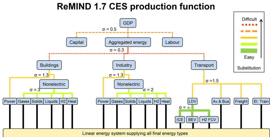
Figure A5. CES production function of the REMIND 1.7 model. Nested CES (constant elasticity of substitution) production functions determine the substitution of production factors, sector-specific energy demands, and energy carriers in the different levels of the function. The macro-economic production function is calibrated for consistency with historic trends; i.e. this specifically includes assumptions about future improvements of the productivity of input factors. Final energy in the baseline scenarios (without climate change) for different sectors is calibrated to projections from the EDGE2 (Energy Demand Generator version 2) model (Levesque et al., 2018).
