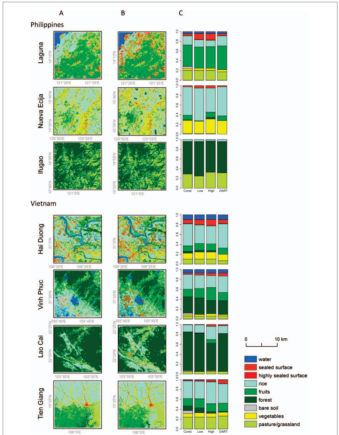
Figure 2. Land use classes in the seven study areas. (a) Observed land use class, (b) land use in 2030 in the expert scenario ‘High-conversion’ and (c) fraction of land use categories in 2030 in all land use change scenarios (Low-conversion, High-conversion and DART). The land use scenario ‘Const’ refers to the observed land use. Highland sites are Lao Cai (VN_3) and Ifugao (PH_3). Lowland sites are Laguna (PH_1), Nueva Ecija (PH_2), Hai Duong (VN_1), Vinh Phuc (VN_2) and Tien Giang (VN_4).
