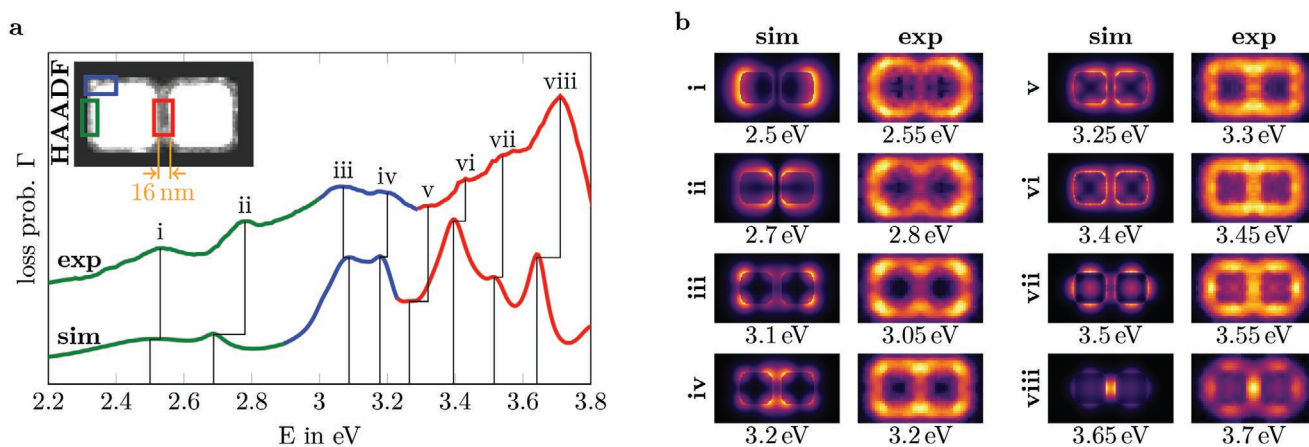
Figure 4. a) Experimental and simulated EEL spectra for a Au@Ag-cube dimer coated with 8 nm silica. Here, the color of the curve corresponds to different spatial sub-areas of the EELS scan, over which the loss probability is averaged. The different sub-areas are indicated by the red, blue, and green rectangles in the high angular dark field (HAADF) image of the dimer. b) EEL probability maps of the modes indicated (i–viii) in (a) respectively. The enhanced coupling of the LSP modes mediated by the silica coating results in a hybridization of the modes excitable in the single NPs, respectively. Note that the experimental obtained EEL probability maps are symmetrized with respect to the central plane of the dimer in order to enhance the signal to noise ratio.
