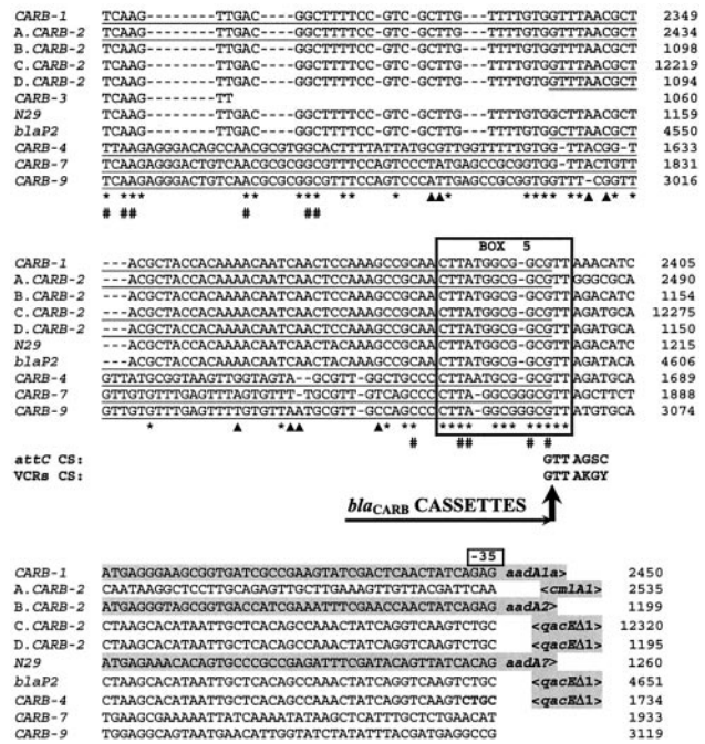
FIG. 3. Flanking regions of bla CARB genes. Relevant features of compared sequences are in Table 1. Numbers on the left correspond to nucleotide positions in the GenBank reports. Gaps (dashes) were introduced in order to maximize the alignment (Clustal X). Codifying regions are signaled by shaded boxes, and the names of corresponding genes are indicated. The 5' and/or 3' ends not included in the alignment are represented by < and >, respectively. cmp, complementary sequence. The truncated codifying sequence ( aadA ?) at the end of N29 shared 97% identity with the integron-encoded gene aadA10 from the P. aeruginosa plasmid R388-R151 (GenBank accession no. U37105). Promoter (Pr) regions (−35 and −10) and the RBS reported previously are shown in boldface, and those identified in this work (the BPROM program, http://www.softberry.com/berry.phtml?topic = promoter ) are additionally underlined. For clarity, VCRs and reported attC elements (underlined sequences) were defined from the third nucleotide upstream to the motif TAAC in the ICS, up to the G in the GTT of the CS. Consensus sequences for both ICS and CS are shown below the alignment. The identities among all available sequences (*) and positions highly conserved among Vibrio repeated sequences (VXR; #) (24) are indicated. The regions of highest identity are boxed (boxes 1 to 5). Changes between the VCRs associated with bla CARB-7 and bla CARB-9 are signaled (▲). Horizontal arrows indicate the boundaries of the bla CARB cassettes (5' to 3'), and vertical arrows indicate the putative recombination points (between G and T in the GTT of the CS).
