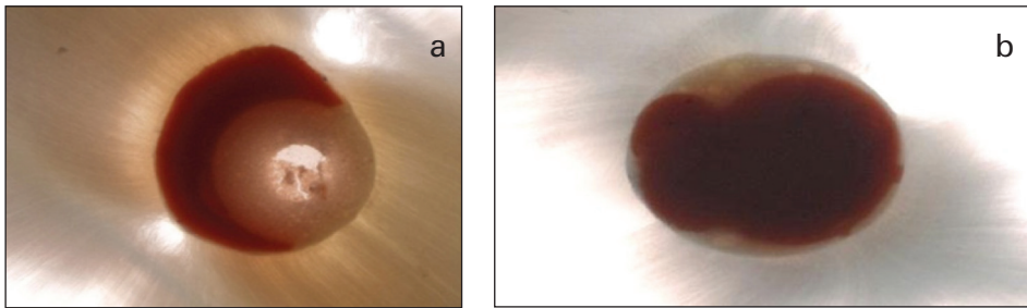
Fig. 8: (a) Massive amount of sealer and the central void; (b) Unsoftened cones.
