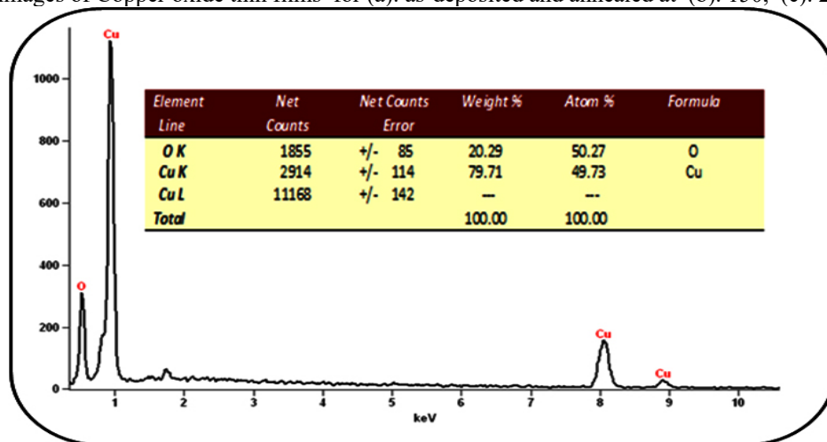
Fig. 7: EDAX Spectrum of Cu 2 O thin films with annealed at 250°C.
