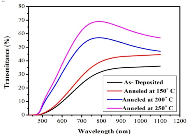
Fig.2: Transmittance spectrum of as-deposited and annealed Copper oxide thin films.
