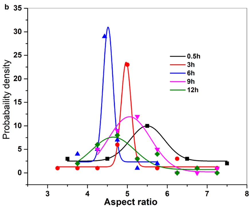
Fig. 9 TEM images a and aspect ratio probability densities b for nanorods with changing hydrothermal time from 0 to 12 h (APTMS is 0.05 g, \text{Fe}^{3+}/\text{Fe}^{2+} = 2:1 )
