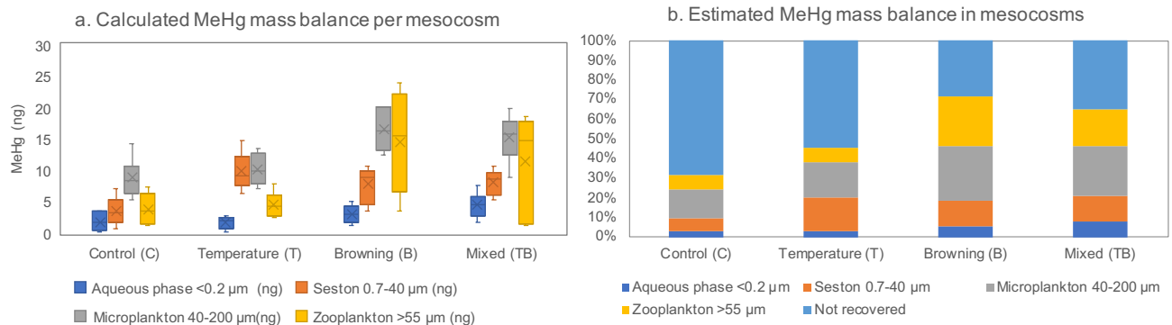
Figure 3. Estimated MeHg mass balance per mesocosm (a) and MeHg distribution across aqueous and biological phases (b) across treatments based on average estimations. Aqueous phase (dark blue), seston (orange), microplankton (grey), and zooplankton (yellow). “Not recovered” in light blue colours represent the proportion of MeHg that was not retrieved in either aqueous phase or solid phase at the end of the mesocosm experiment.
