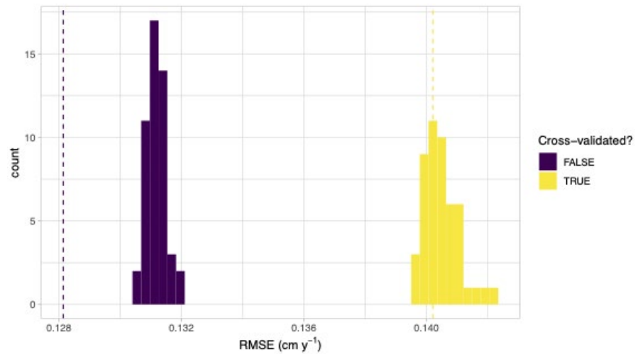
FIGURE 6 Comparison of root mean squared error of models for standard, permuted, and spatially cross-validated error estimates. The dotted lines show observed RMSE while the histograms show the null distribution of RMSE for 49 permutations under the null hypothesis of no competitor species identity effects. The colors indicate whether spatial cross-validation was used or not
