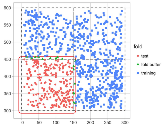
FIGURE 5 Schematic of spatial cross-validation. Using the k = 1 fold (bottom-left) as the test set, k = 2 through 4 as the training set, along with a fold buffer extending outward from the test set to maintain spatial independence between it and the training set
