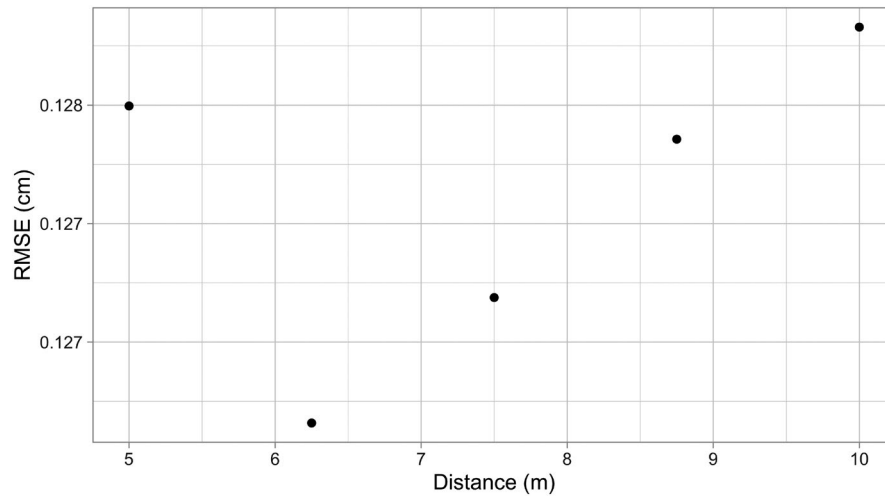
FIGURE 7 Cross-validated RMSE estimates for 5 competitive distances
