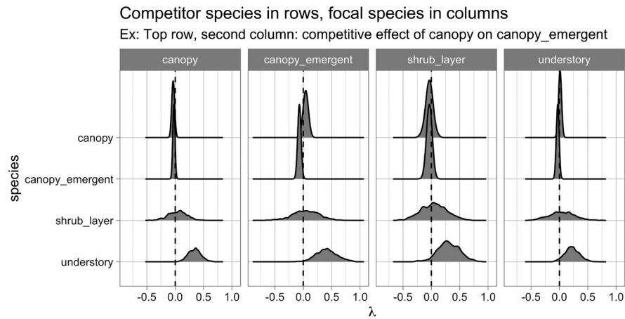
FIGURE 8 Posterior distributions of all competition parameters
