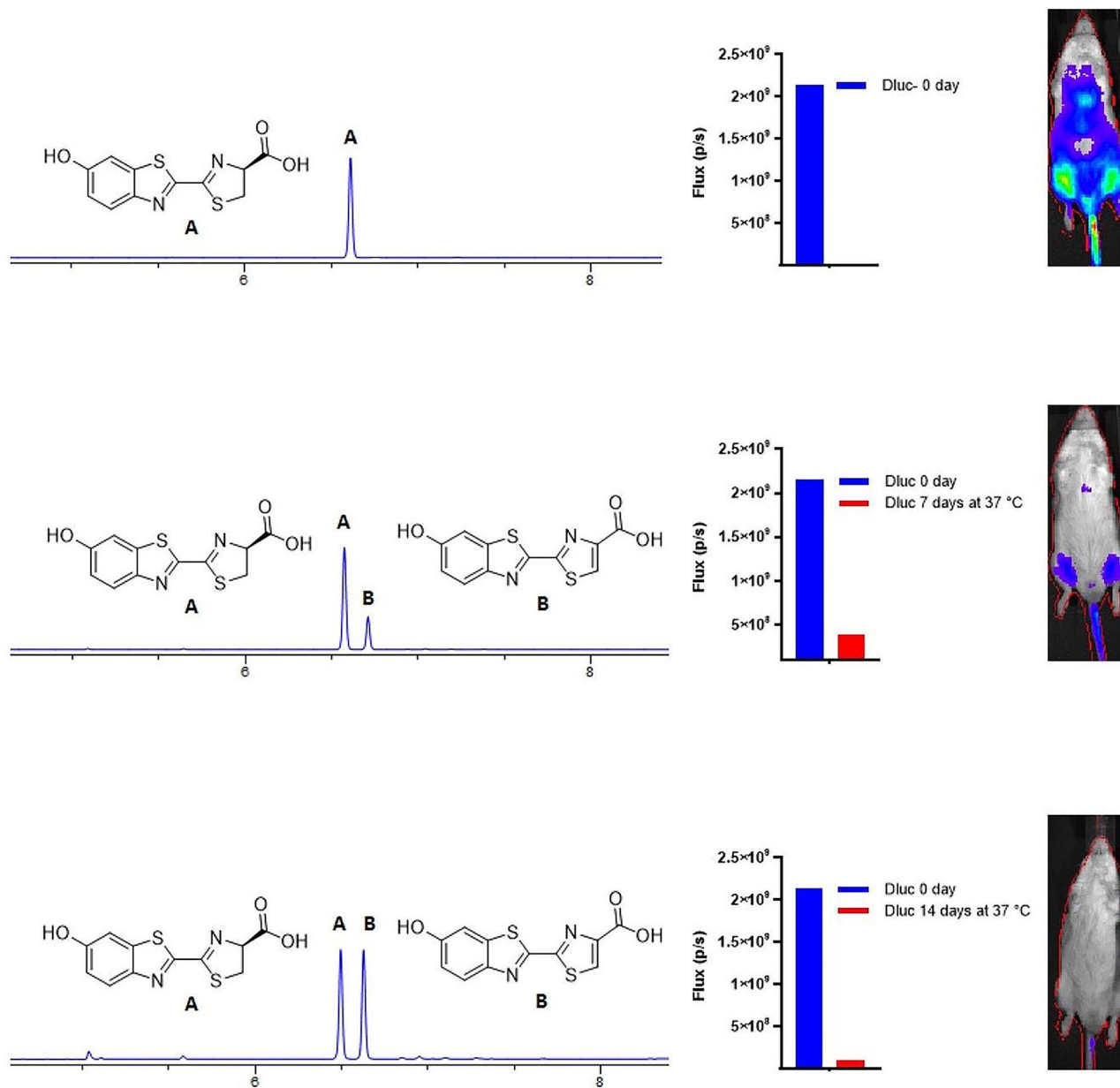
Figure 7. Evaluation of D-luciferin after incubation at body temperature. Liquid chromatography / mass spectrometry (LC/MS) and in vivo bioluminescence imaging with D-luciferin incubated in aqueous buffer at 37 °C for 0, 7, or 14 days. FVB/NJ mice received intravenous injection of AAV9-CMV-WTluc2 as previously described in a method that primarily transduces heart and leg muscles (Mofford et al., 2015) and images were collected 12 min postinjection (ip) of the D-luciferin solution. Images shown are from one male mouse imaged on different days, and the 0-day data from this mouse are shown for comparison with the 7- and 14-day data on the lower two histograms.
