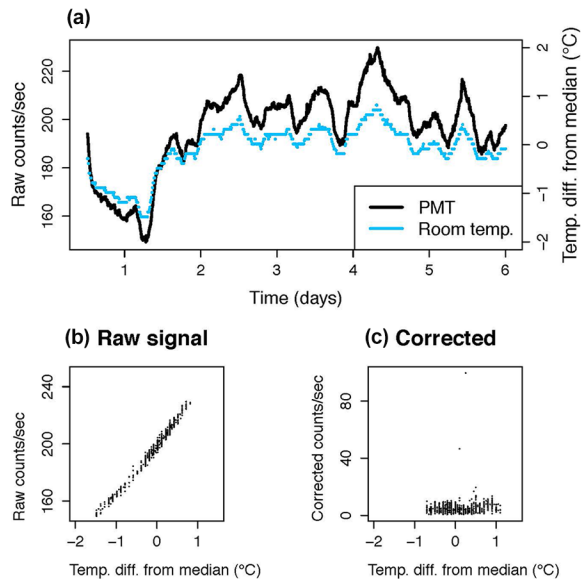
Figure 1. Fluctuations in room temperature impact photomultiplier (PMT) output, as shown in a recording from an empty recording chamber with no animal present over 5 days with extreme temperature variations. This is corrected by subtracting dark counts in the LumiCycle In Vivo (Actimetrics) as shown in (c). (a) Raw photomultiplier tube output (black line) tracks room temperature (shown in blue dotted line) prior to adding the capability for dark count subtraction. (b) Same data as in (a) plotted to demonstrate the tight correlation. (c) Following installation of software to collect background readings every 15 min and subtract these from prior PMT outputs, effects of room temperature fluctuations are corrected (compare [c] to [b]). Abbreviation: PMT = photomultiplier tube.
