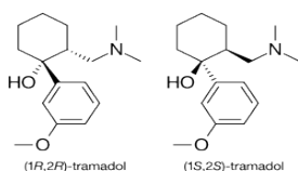
Fig. 2: Structure of tramadol hydrochloride [4]
