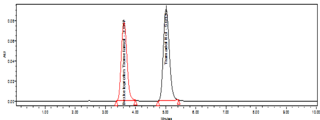
Fig. 3: Optimized chromatogram
