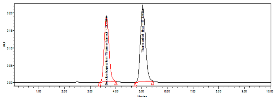
Fig. 14: Chromatogram for linearity 80%
