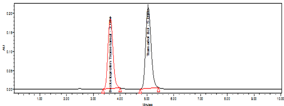
Fig. 13: Chromatogram for linearity 70%
