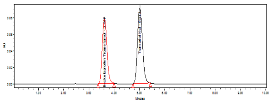
Fig. 15: Chromatogram for system precision-1
