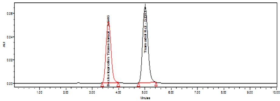
Fig. 8: Chromatogram for linearity 20%
