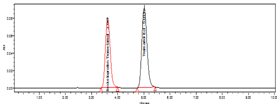
Fig. 19: Chromatogram for system precision-5
