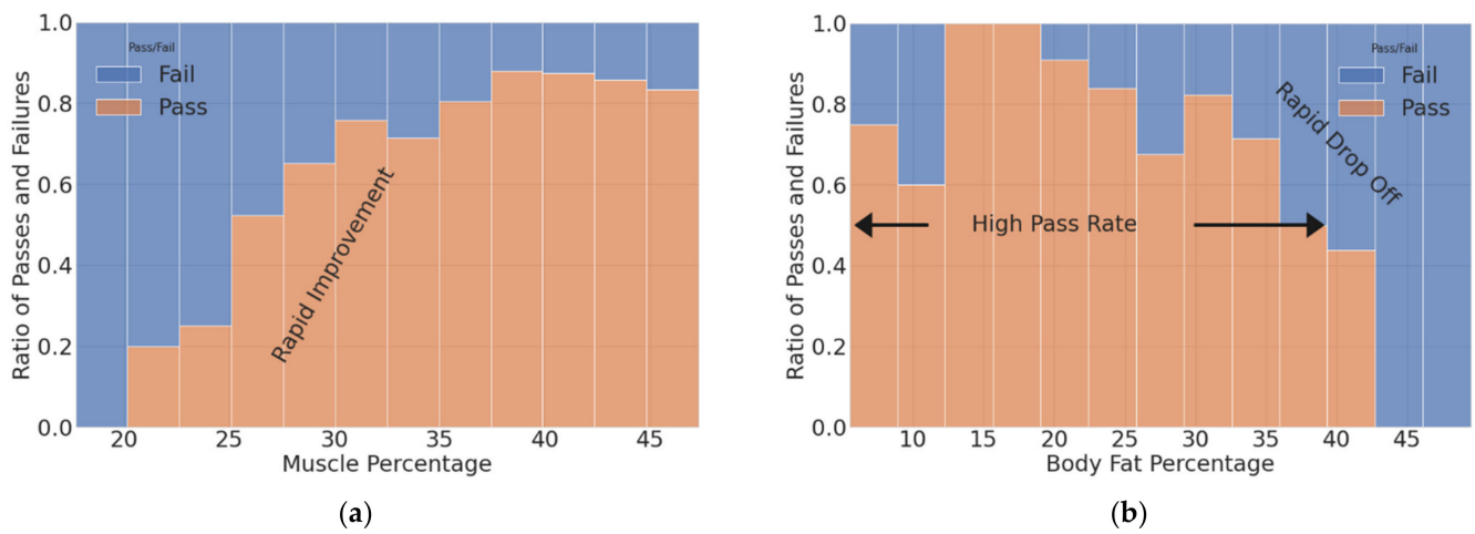
Figure 2. Graphical analysis of the ratio of passing/failing the APFT vs. (a) muscle percentage and (b) body fat percentage.
