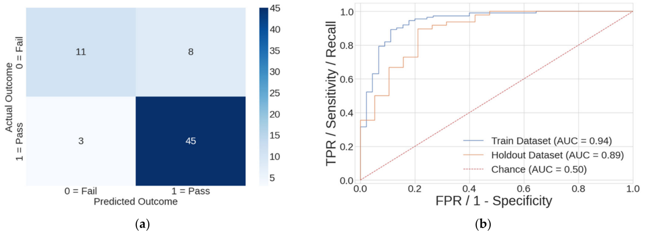
Figure 4. Performance graphs for the best ( four-feature p-value ) classical logistic regression model. (a) the confusion matrix resulting from the holdout dataset, where APFT Failure = 0 and APFT Pass = 1. (b) ROC curves from the training dataset, holdout dataset, and trivial Chance model. TPR: True positive rate; FPR: False positive rate.
