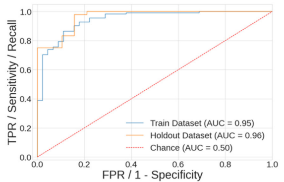
(c2) Limited Model ROC Curves
