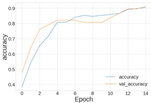
(b1) Full Model Training Curves
