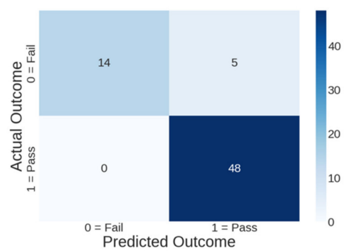
(d2) Limited Model Confusion Matrix
