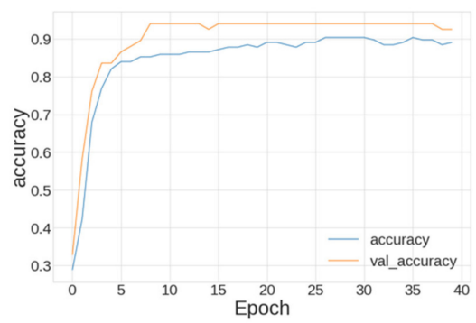
(b2) Limited Model Training Curves
