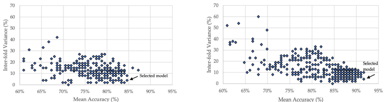
Figure 5. Families of models from the multidimensional hyperparameter sweeps on the full dataset (left), and the limited dataset (right). On each subfigure, an arrow indicates the best model.
