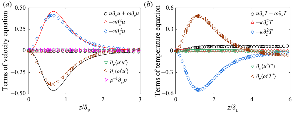
Figure 5. (a) Contributions of the mean convection term u\partial_x u + \omega\partial_z u , molecular momentum diffusion components -v\partial_x^2 u and -v\partial_z^2 u , Reynolds stress gradient components \partial_x\langle u'u' \rangle and \partial_z\langle w'u' \rangle , and pressure gradient 1/\rho\partial_x p , as a function of the normalised vertical distance z/\delta_v . The unit of the terms is U_f^2/H . The two solid lines show the calculated terms of the velocity equation using the analytical solution \tilde{u}(\xi) in (4.14) with a = 1.19 . (b) Contributions of the mean convection term u\partial_x T + \omega\partial_z T , molecular thermal diffusion components -\kappa\partial_x^2 T and -\kappa\partial_z^2 T , and turbulent heat flux gradient components \partial_x\langle u'T' \rangle and \partial_z\langle w'T' \rangle , as a function of z/\delta_v . The unit of the terms is U_f\Delta T/H . The DNS data used for the calculations shown in (a) and (b) are obtained at Pr = 0.17 and Ra = 1 \times 10^9 in a vertical thin disk with \Gamma = 0.2 .
