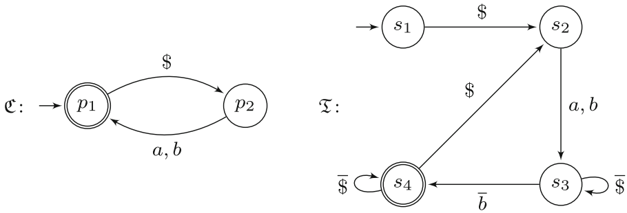
Fig. 2 NFAs \mathcal{C} and \mathcal{T} accepting LW^* and (W\bar{R})^* , respectively, from Example 5.7
