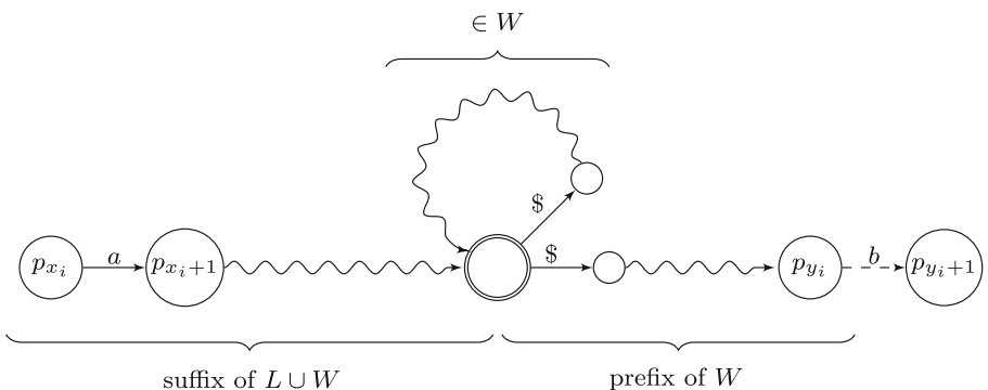
Fig. 1 A run labeled with v_i from p_{x_i} to p_{y_i} in \mathcal{C}
