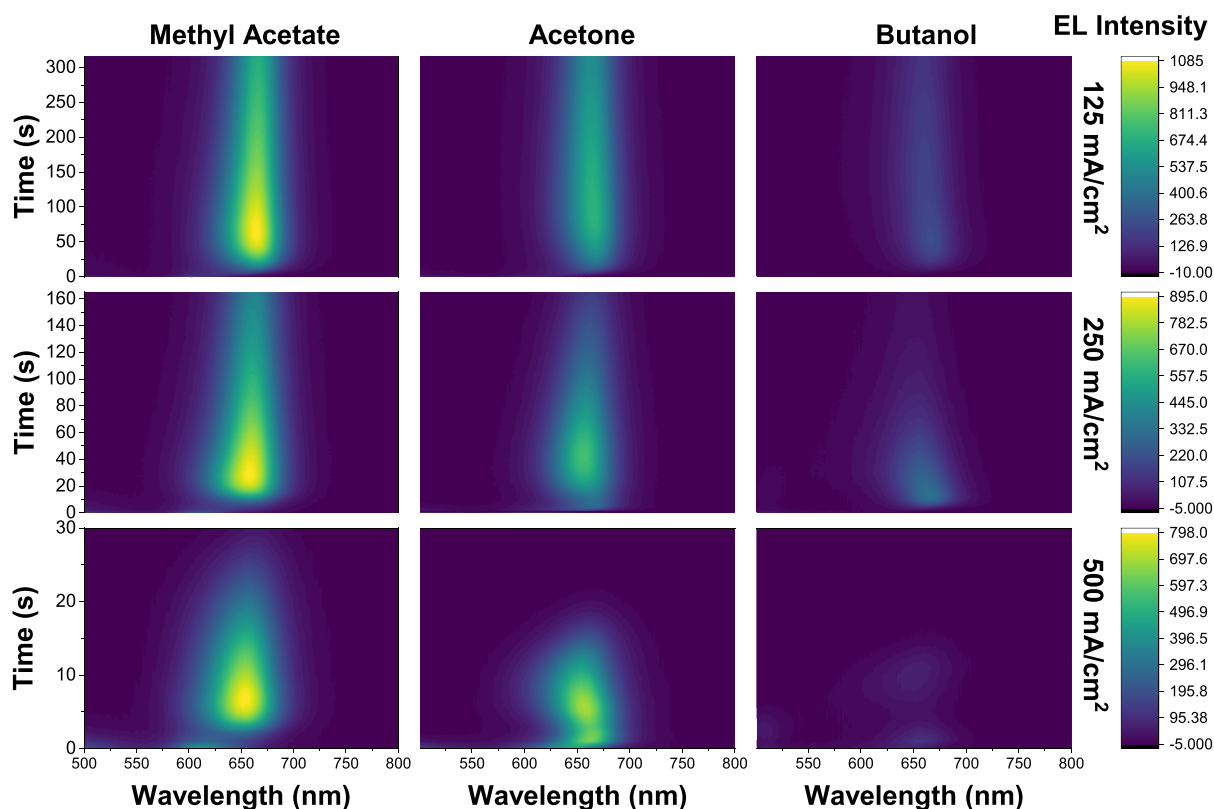
Figure 6. Electroluminescence stability of the purified NC-based LEDs, in which the CsPbBr x I 3-x NCs were purified using methyl acetate, acetone, or butanol antisolvents.
