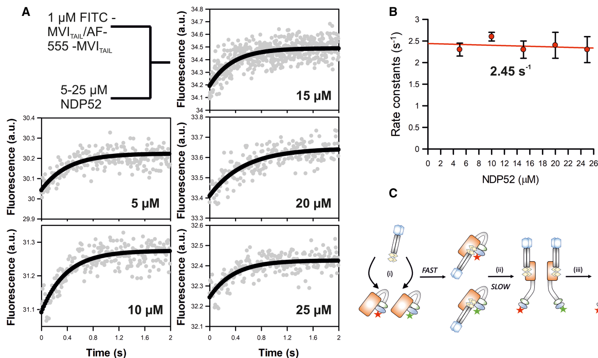
Figure 4. Binding partner driven dimerization of Myosin VI.
