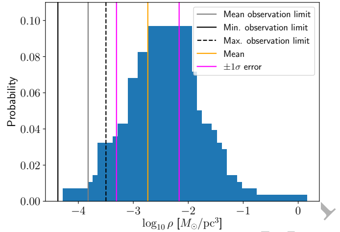
Figure 6. The distribution of each dwarf galaxy's mean baryonic density \rho within its half-mass radius. The orange vertical line shows the sample mean, while the magenta lines offset by \pm 0.57 dex show the standard deviation around it. The grey line shows the density of a dwarf corresponding to the observational surface density detection limit of \Sigma_{\min} = 0.26 M_{\odot}/\text{pc}^2 assuming the mean M/L_{r'} = 1.10 and mean \rho/\Sigma = 0.59 \text{ kpc}^{-1} . If instead we add (subtract) the standard deviations in the M/L_{r'} ratios, we have that \Sigma_{\min} = 0.35 (0.17) M_{\odot}/\text{pc}^2 . From these and by adding (subtracting) the standard deviations in the \rho/\Sigma relation, we obtain the \rho value given by the dashed (solid) black line.
