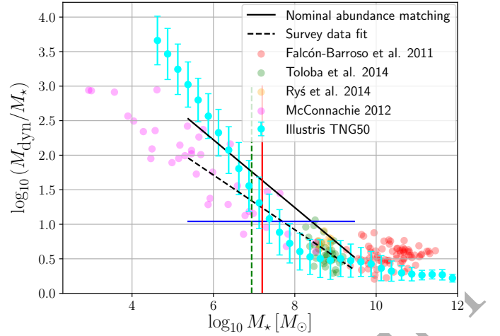
Figure 16. The relation between stellar mass and Newtonian dynamical mass (Equation 64). The semi-transparent coloured dots represent galaxies from four different galaxy surveys as indicated in the legend (Falcón-Barroso et al. 2011; McConnachie 2012; Ryś et al. 2014; Toloba et al. 2014). The cyan dots with error bars represent the logarithmic mean and dispersion of the total/stellar mass ratio within the stellar r_h of the dwarfs in each M_* bin in the \Lambda CDM cosmological simulation Illustris TNG50 (Pillepich et al. 2018, 2019; Nelson et al. 2019a,b). These bins have a width of 0.25 dex and cover the mass range \log_{10}(M_*/M_\odot) = 4.5 - 12 . The solid black line represents the expected trend in \Lambda CDM with the nominal dark matter fraction from abundance matching (Equation 10). The dashed black line represents the fit to the dwarfs from the aforementioned galaxy surveys in the mass range covered by the FDS dwarfs. The horizontal blue line at \log_{10} 11 shows our conservative assumption that M_{\text{DM}} = 10 M_* . In these three cases, the relations are only plotted over the M_* range of the FDS dwarfs. Their median mass is shown with the dashed green vertical line. The solid red vertical line corresponds to the stellar mass below which core formation is inefficient in \Lambda CDM (see the text).
