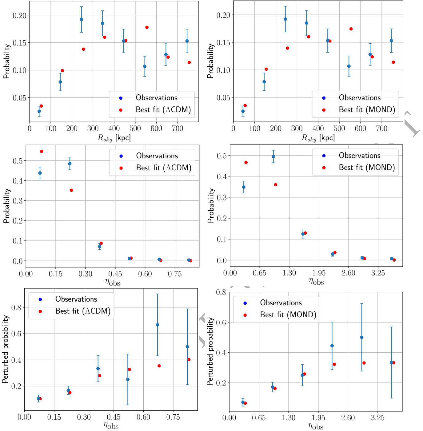
Figure 9. Comparison between observations and the best-fitting simulation in \Lambda CDM (left column) and MOND (right column) in terms of the distribution of projected separation R_{\text{sky}} from the cluster (first row), tidal susceptibility \eta_{\text{obs}} (second row), and likelihood that a dwarf appears disturbed as a function of \eta_{\text{obs}} (third row). The observations (blue points with error bars) and the best-fitting simulation in each theory (red points) are plotted at the centre of each bin, but dithered slightly along the x -axis for clarity in case the model works well. The bin width in R_{\text{sky}} is 100 kpc in both theories. For \eta_{\text{obs}} , the bin width is 0.15 in \Lambda CDM and 0.65 in MOND.
