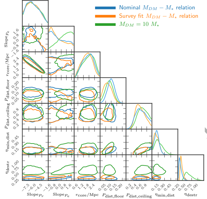
Figure F1. Triangle plot showing the inferred parameter values in the \Lambda CDM model constrained by our statistical analysis with the nominal dark matter fraction (Equation 10; blue), our fit to the empirically determined dark matter fractions of nearby isolated dwarfs (Equation 65; orange), and a very conservative case assuming that the mass of dark matter within the optical radius of each dwarf is only 10\times that of the baryons (green).
