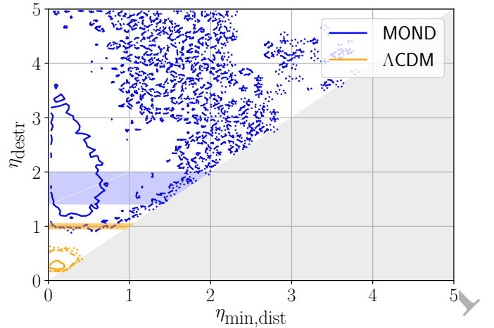
Figure 14. Joint inference on \eta_{\text{min,dist}} and \eta_{\text{destr}} (Section 5.2.4). We show the 1\sigma (inner solid line), 3\sigma (dashed line), and 5\sigma (outer dotted line) confidence region for MOND (blue) and \Lambda CDM (orange). The thick orange line shows the \Lambda CDM expectation that \eta_{\text{destr}} \approx 1 . For MOND, the corresponding expectation from our N -body simulations (Section 7) is that \eta_{\text{destr}} = 1.70 \pm 0.30 (horizontal blue stripe). The grey shaded region below the line of equality is not allowed by our choice of prior because it is unphysical.
