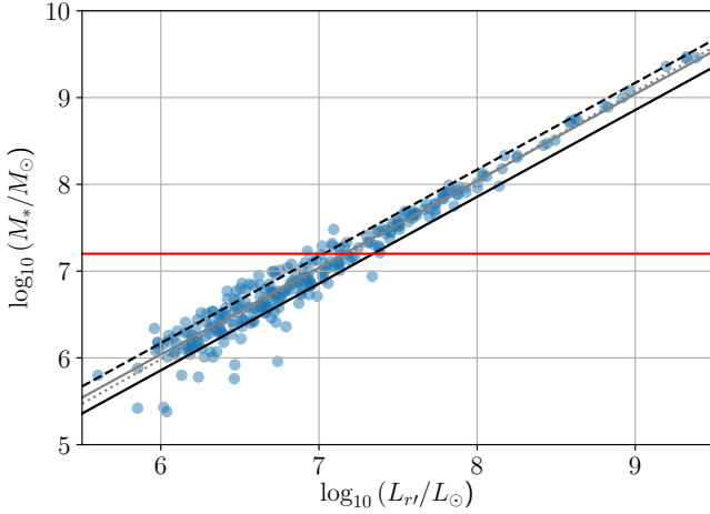
Figure 7. The relation between mass and luminosity in the r' -band for the non-nucleated sample of dwarfs in the FDS catalog, with both shown on a \log_{10} scale. The assumed M/L ratios are based on empirical relations with the colour (Section 2). The dotted grey line shows the linear regression, while the solid grey line shows our adopted fit assuming a slope of 1. The dashed (solid) black line shows one standard deviation above (below) the mean M_*/L_{r'} . The horizontal red line at 10^{7.2} M_\odot shows the stellar mass below which core formation is inefficient in \Lambda CDM (Section 8).
