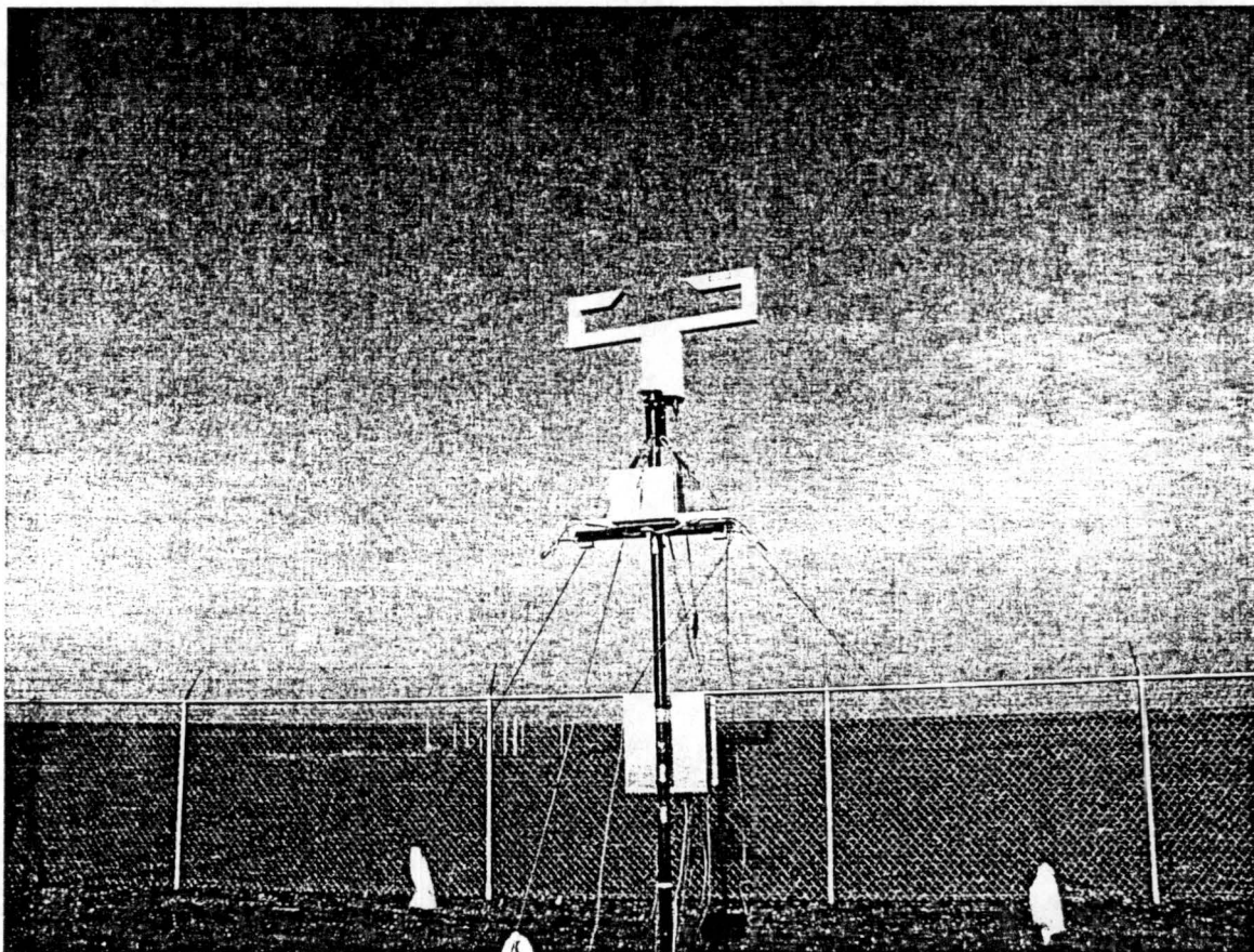
Figure 3.6 Gerber Scientific PVM 100 and CSU Optical Fog Detector at main site in Angiola, CA.
