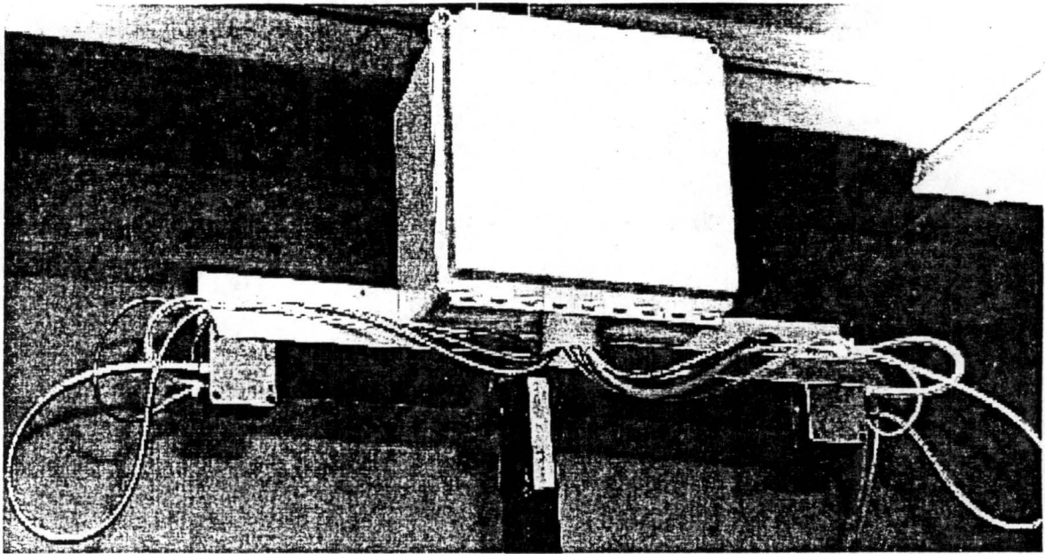
Figure 3.1 CSU Optical Fog Detector shown in the laboratory mounted on a 3-meter pole.
