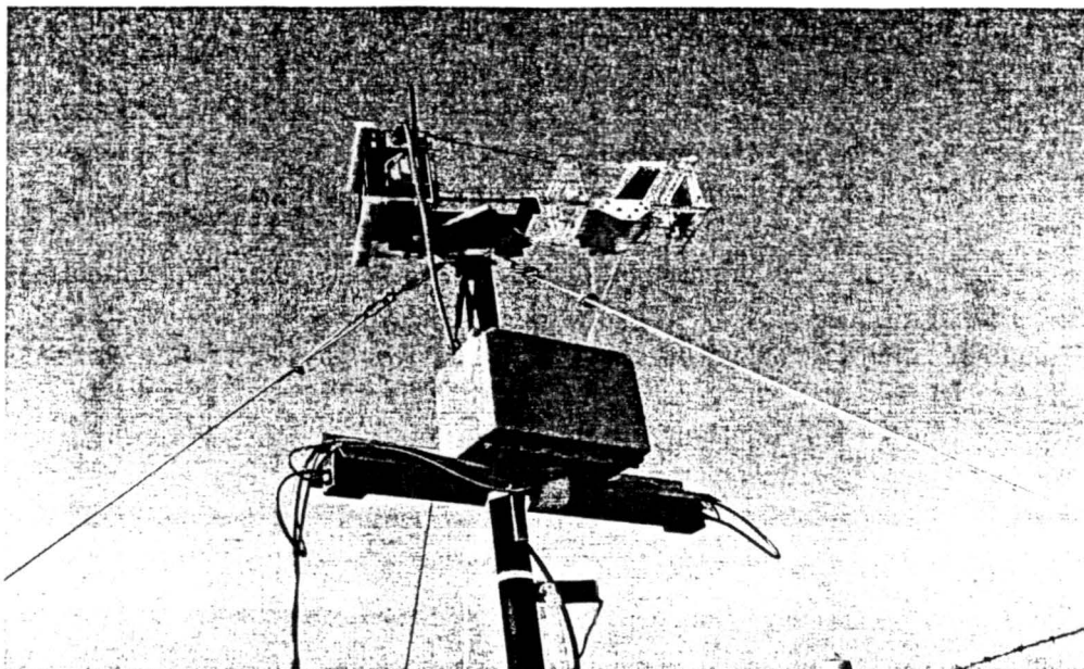
Figure 3.2 Setup of CSU Optical Detector and CASCC2 at Helm, CA.
