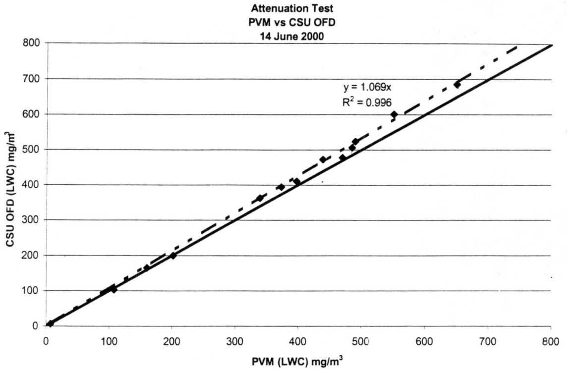
Figure 2.15b. One to one results from first attenuation test shows a very high linear correlation between the CSU OFD and the PVM.
