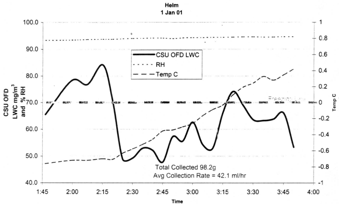
Figure 3.12 Event from Helm, CA. January 1, 2001
