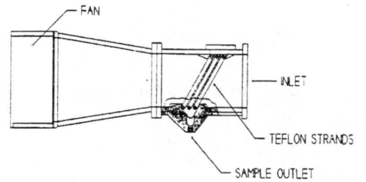
Figure 3.4 The CASCC2 collects bulk cloudwater samples (from Demoz et al., 1996).
