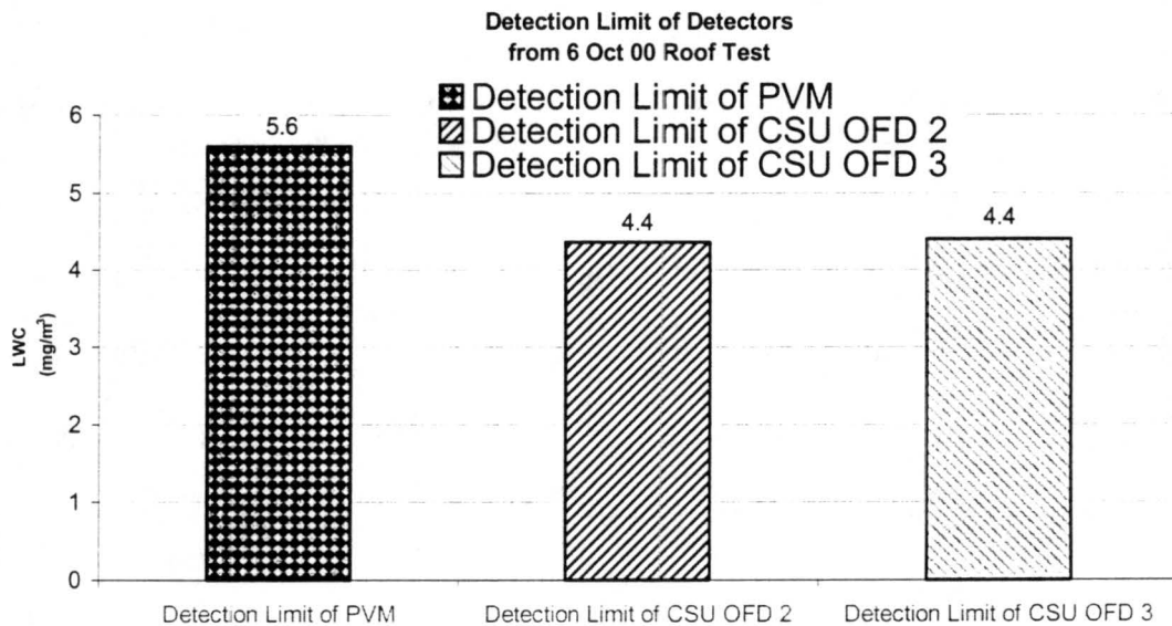
Figure 2.28. Calculated detection limit (signal to noise ratio) of PVM and the CSU OFD.
