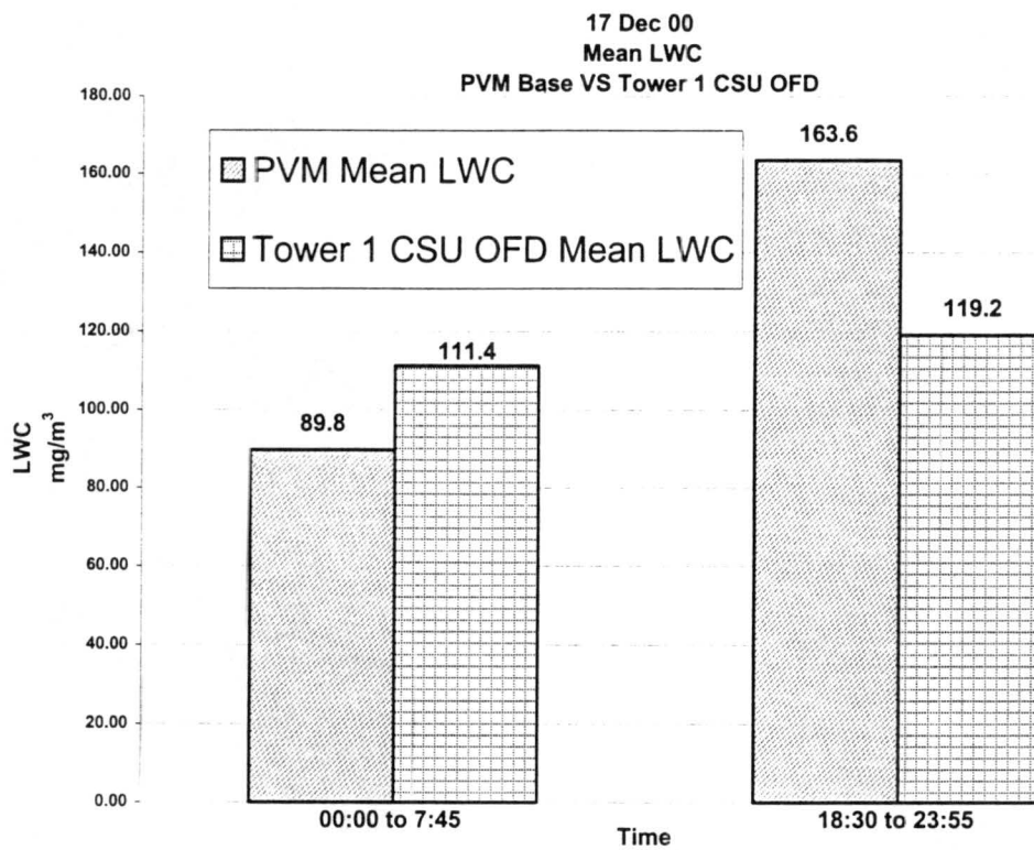
Figure 3.18 Mean LWC values from PVM and CSU OFD Tower Level 1, December 18, 2000
