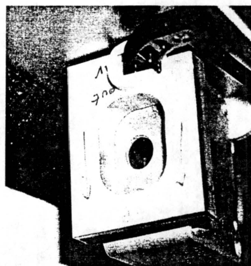
Figure C.4 Proper placement of calibration disk for SPAN adjustment.
