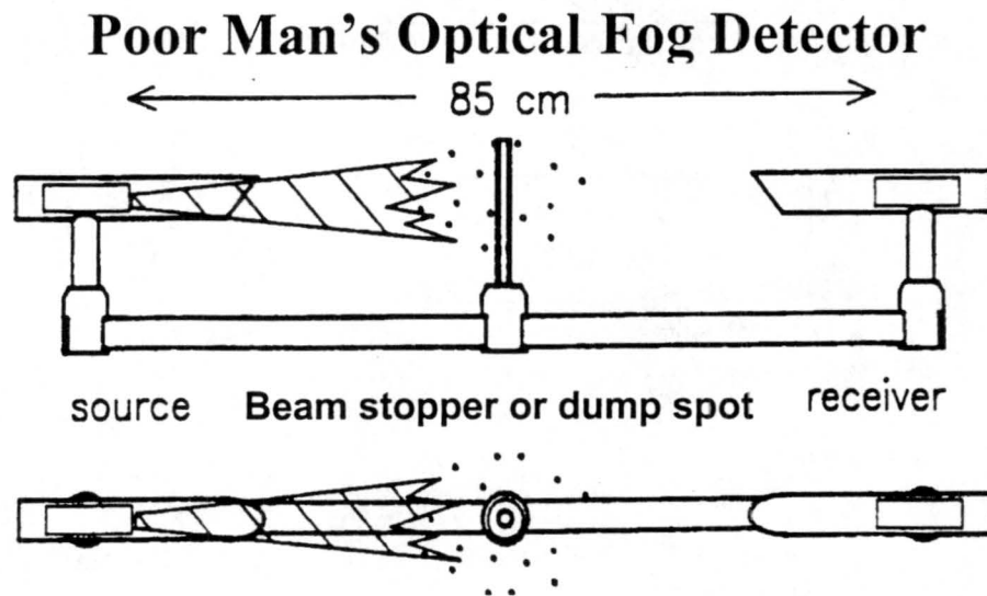
Figure 1.8 ECN's OFD (Mallant, 1990).
