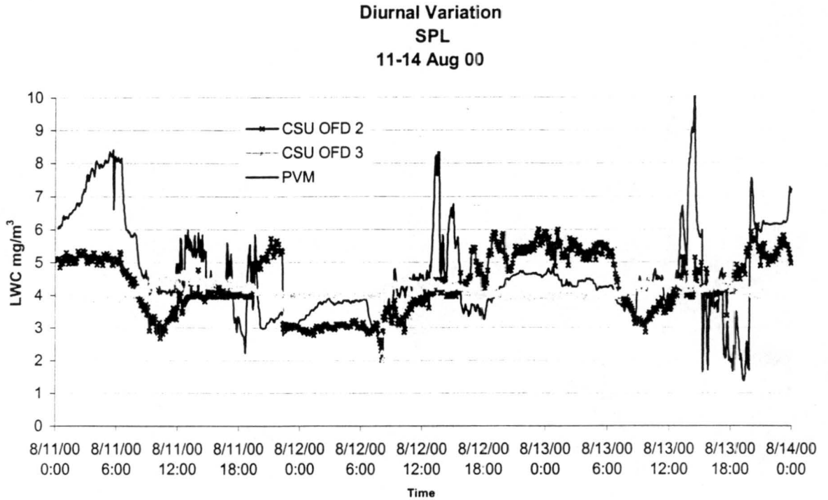
Figure 2.25. Diurnal variation test.
