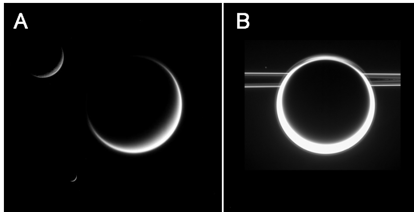
Figure 6. (A) This photograph taken by the Cassini space probe of Saturn’s moons Rhea (upper left), Titan (center) and Mimas (lower left) illustrates the role that Titan’s atmosphere plays in changing the illumination of the moon when almost backlit. The illuminated arc is much brighter and more extensive on Titan due to refraction and forward scattering through its significant atmosphere. (B) In the image on the right, Titan is seen in the foreground with Saturn’s rings in the background. Both are backlit in this image, and Titan is surrounded by a brilliant halo of refracted light. Public Domain Images. Credit: NASA/JPL-Caltech/Space Science Institute.
