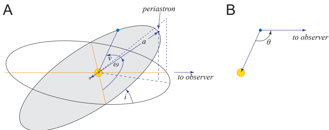
Figure 2. (A) An illustration of the anatomy of a typical Keplerian orbit. The planet moves on an elliptical orbit with the star located at one focus. The semi-major axis, a , of the ellipse is used to characterize the star-planet distance. The argument of the periastron, \omega , is the angle describing how the periastron (point of closest approach) is rotated with respect to the observer. The true anomaly, \nu , describes the position of the planet along the orbit in the frame of the host star with the origin at the periastron. (B) The angle \theta(t) indicates the orbital phase, which is defined as the angle between the planet-star vector and the planet-Earth vector.
