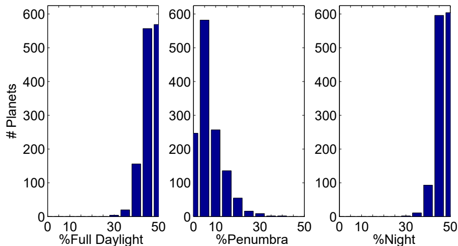
Figure 5. For 1306 exoplanets in the Exoplanet Archive, this figure shows histograms of the percent of the surface area that is in full daylight, in a penumbral zone and in completely dark night. Note that slightly less than half of the planets have a 50% full daylight zone or a 50% night zone. It is most common for planets to have a 5% penumbral zone, and more than one quarter of the planets have penumbral zones that are larger than 5%. There are four planets with significant penumbral zones in which the full daylight zone covers only about 30% of the surface of the planet.
