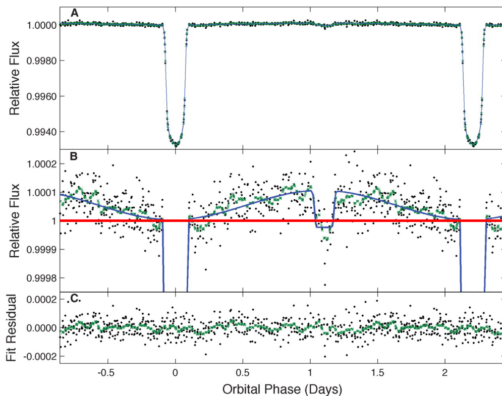
Figure 3. (A) Light curve of HAT-P-7b recorded by Kepler as processed and published by Borucki et al. [26] (reprinted here with permission). (B) The same light curve at greater magnification. The red line marks the baseline flux. The plot in (C) illustrates the residual, which is the difference between the data and the model. The lack of obvious structure in the residual indicates that most of the effects have been well modeled.
