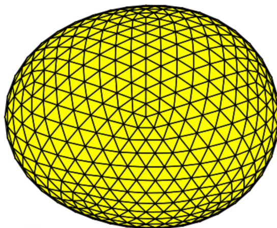
Figure 7. This is an exaggerated image of a star that has been tidally distorted by a closely-orbiting planet ( \frac{M_p}{M_S} = 9.5425 ). The increased cross-sectional area results in variations in flux that oscillate at twice the orbital period as the planet revolves around the star.
