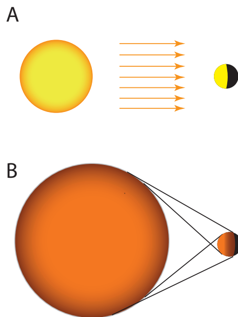
Figure 4. The range of geometries of a planet illuminated by a star. (A) A planet orbits an average star at a great distance. The star's rays are more or less parallel, so that one-half of the planet is illuminated daylight and the other half is in night. (B) A planet in a close-in orbit around a giant star is more than 50% illuminated with a full daylight zone, a penumbral zone and a night zone.
