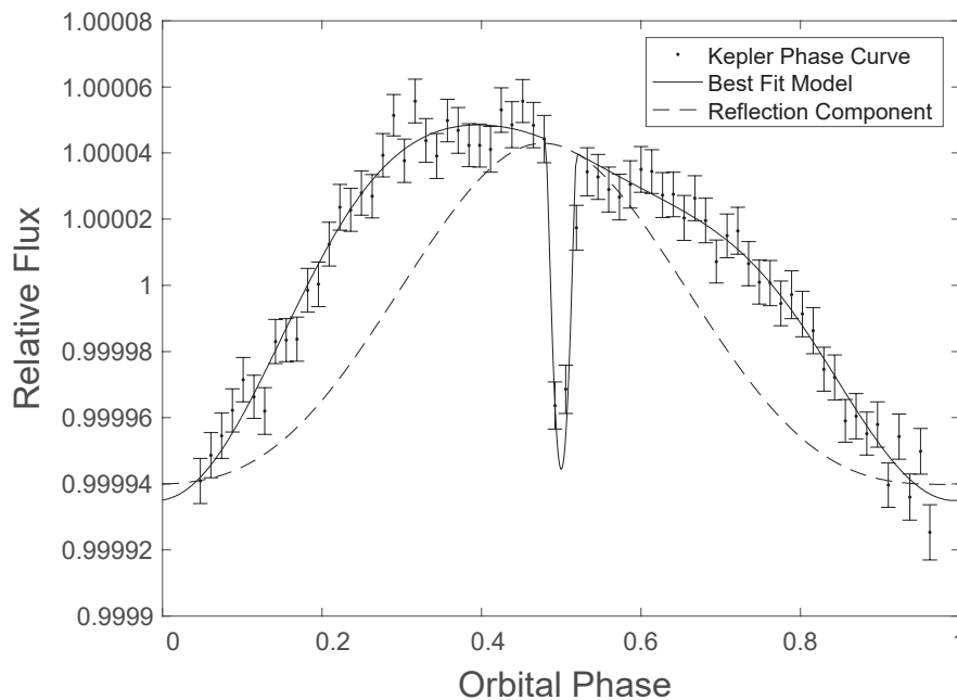
Figure 8. An illustration of the best fit model (REB + SR) for Kepler-76b. The overall shape of the light curve is due to the reflected light, Doppler boosting and ellipsoidal variations. The secondary eclipse can be observed at an orbital phase of 0.5, which is shifted from the peak of the reflected light component (dashed curve) by 8.53^\circ \pm 0.12^\circ , which most likely is due to atmospheric superrotation.
