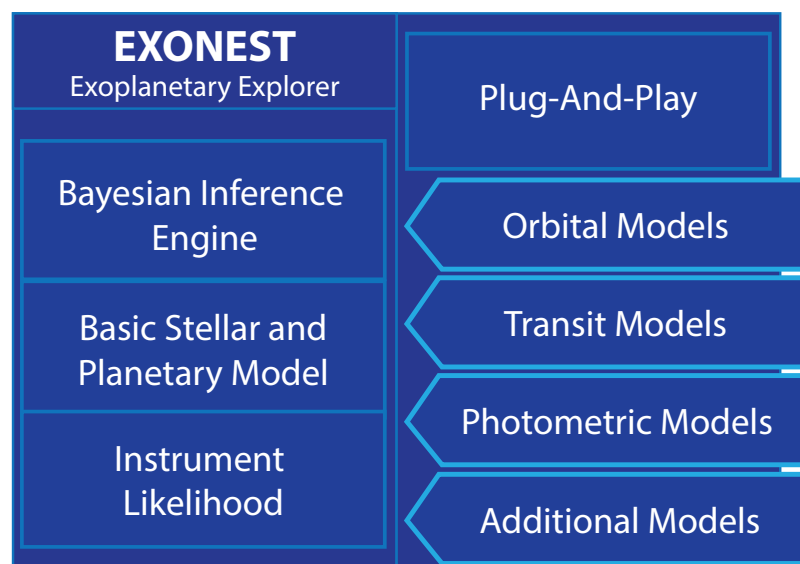
Figure 1. An illustration of the structure of the EXONEST software package.
