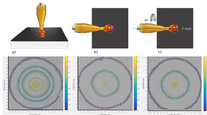
Figure 1. Schematic view of Isodose curves of the 5 cm INTRABEAM™ applicator with corresponding radiation setup. A. The applicator and the probe inside it, placed perpendicularly to the center of an 18 \times 24 \text{ cm}^2 Radiographic film; B. Applicator and the probe parallel to the Radiographic film piece, which the \pm X axis is parallel to the film surface; C. Similar to (B), with 90^\circ rotation around the Z-axis, the \pm Y axis was parallel to the film surface. The setup was carried out in the air with 6 seconds of radiation for each step
