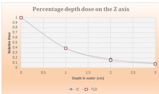
Figure 2. Percentage depth dose on the Z axis. Curves provided using the ion chamber (PTW 23342) and thermoluminescent dosimeters in the water phantom. The ionization chamber (IC) values represent the treatment planning system (TPS) data set
