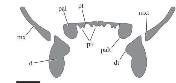
Figure 5. Schematic posterior view cross-section through the snout level of S. leyesi gen. et sp. nov. Scale bar equals 10 mm. d, dentary; dt, dentary teeth; mx, maxilla; mxt, maxillary teeth; pal, palatine; palt, palatine teeth; pt, pterygoid; ptt, pterygoid teeth.
