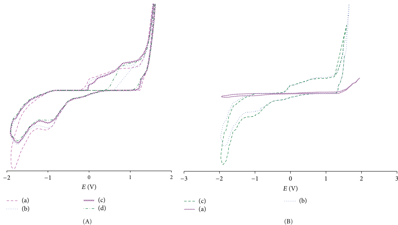
FIGURE 2: Cyclic voltammograms of C1 . Profiles corresponding to: (A) different concentrations of drug in 1% DMSO: (a) 0.014 \mu M ; (b) 0.14 \mu M ; (c) 0.28 \mu M ; and (d) 0.90 \mu M . (B) (a) C1 ; (b) GSH: C1 (1:1); and (c) GSH: C1 (2:1). Experimental conditions were as described in Section 2.
