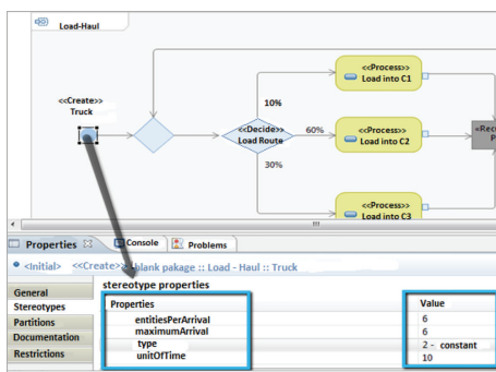
FIGURE 3: Properties of the stereotype <<Create>>.
