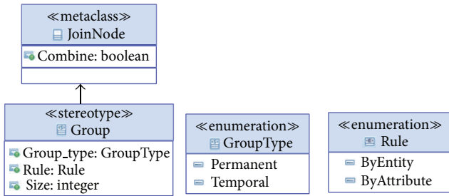
FIGURE 7: Metaclass JoinNode and its corresponding stereotype.
