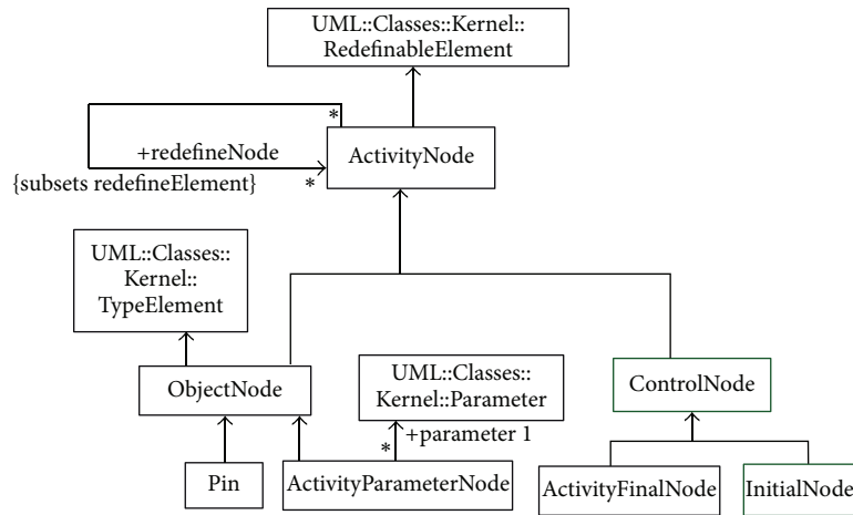
FIGURE 5: Metamodel of the OMG specification.
