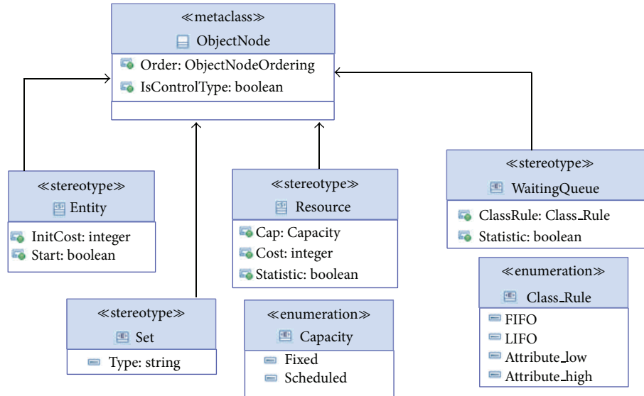
FIGURE 8: The ObjectNode metaclass with its stereotypes.
