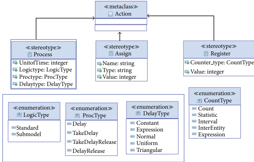
FIGURE 6: The metaclass action and its stereotypes.
