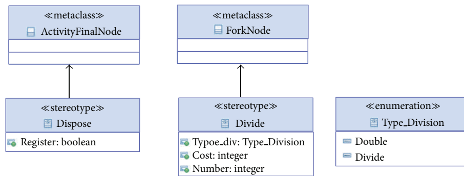
FIGURE 9: Metaclass ActivityFinalNode and ForkNode with its extended stereotypes.
