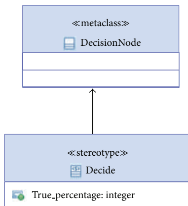
FIGURE 10: The metaclass DecisionNode and its stereotype.
