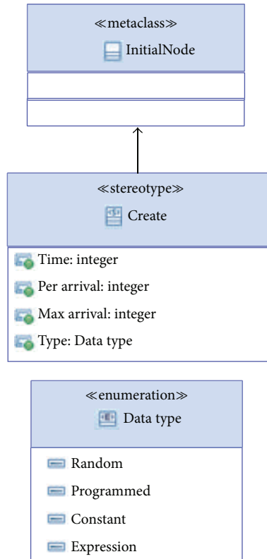
FIGURE 4: Relationship between metaclass and stereotype <<Create>>.
