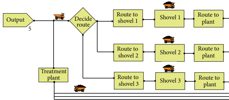
FIGURE 2: Limestone quarry simulation.
