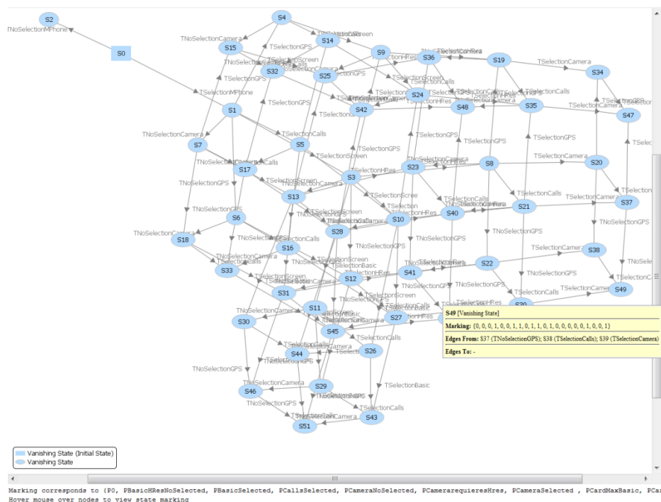
Fig. 9. Partial view of the reachability graph.
