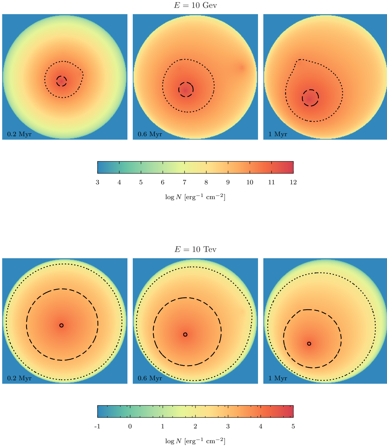
Figure 2. Proton distribution at fixed energy projected along the line of sight for the case \chi = 10^{-1} . Top: E_p = 10 \text{ GeV} ; bottom: E_p = 10 \text{ TeV} . Time evolves from left to right. The level curves correspond to 0.1 (dotted), 1 (dashed), and 10 (continuous) times the CR background distribution.
