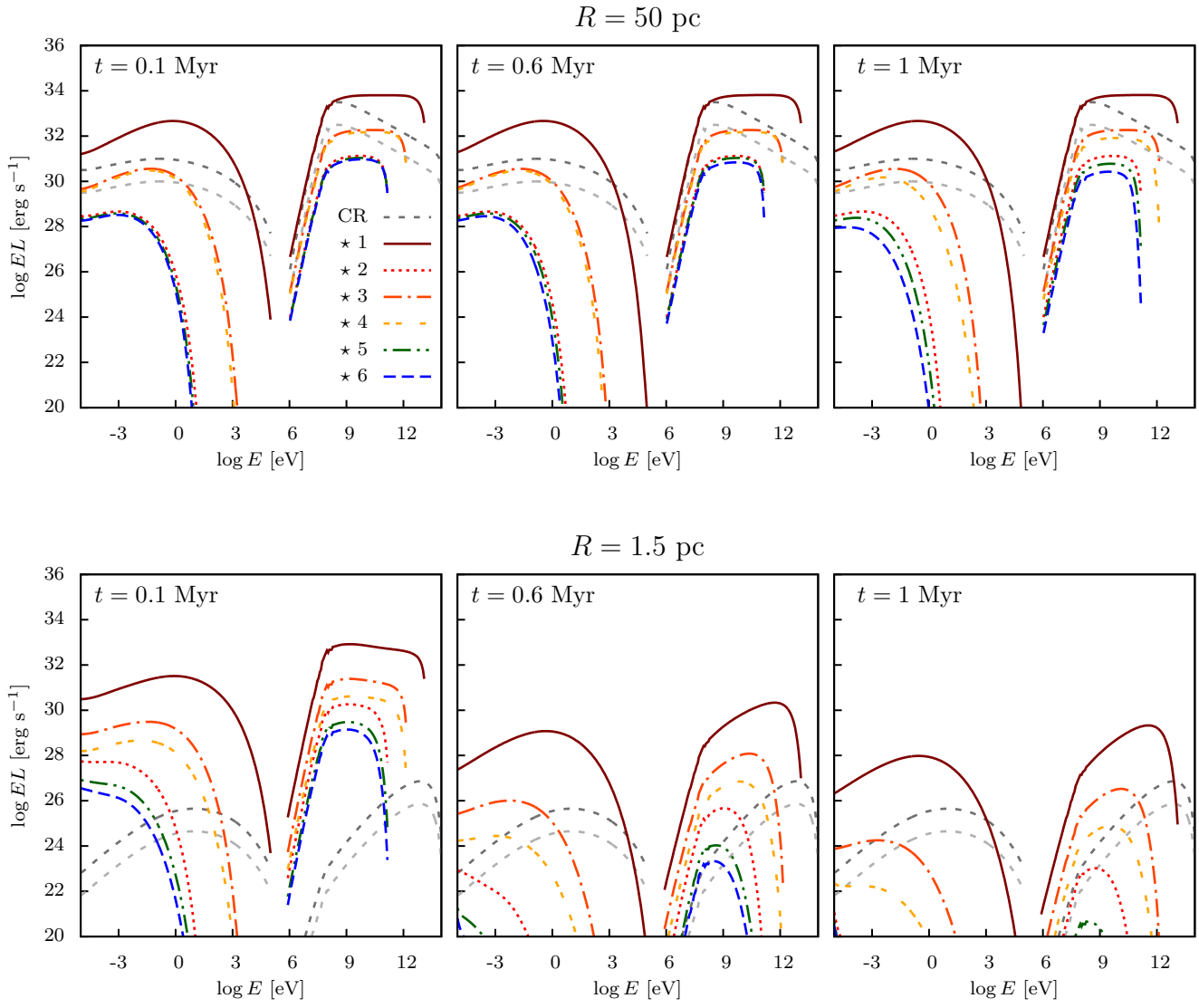
Figure 9. Same as Fig. 8 in the case \chi = 10^{-3} .
