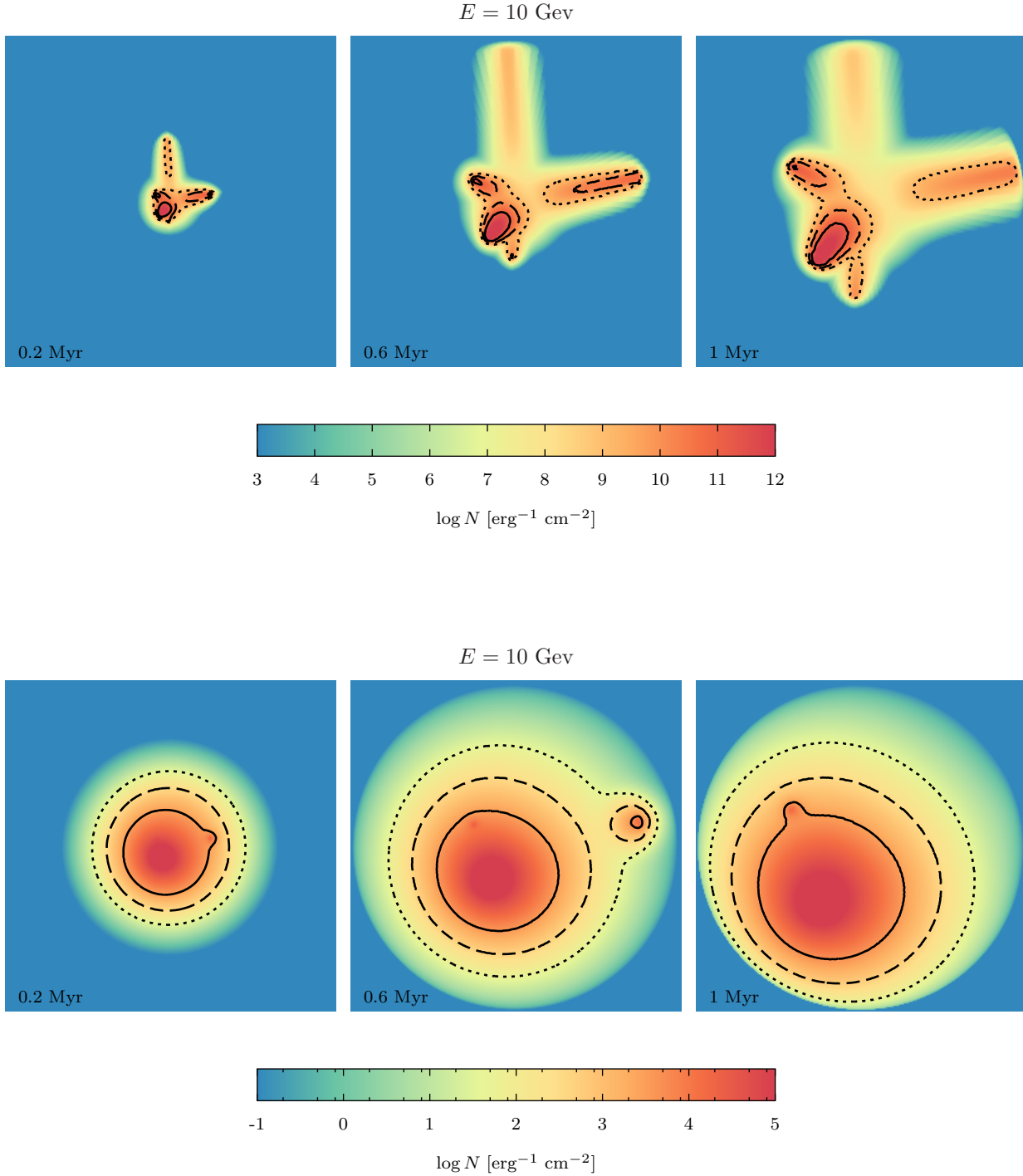
Figure 3. Same as the last figure, for \chi = 10^{-3} .
