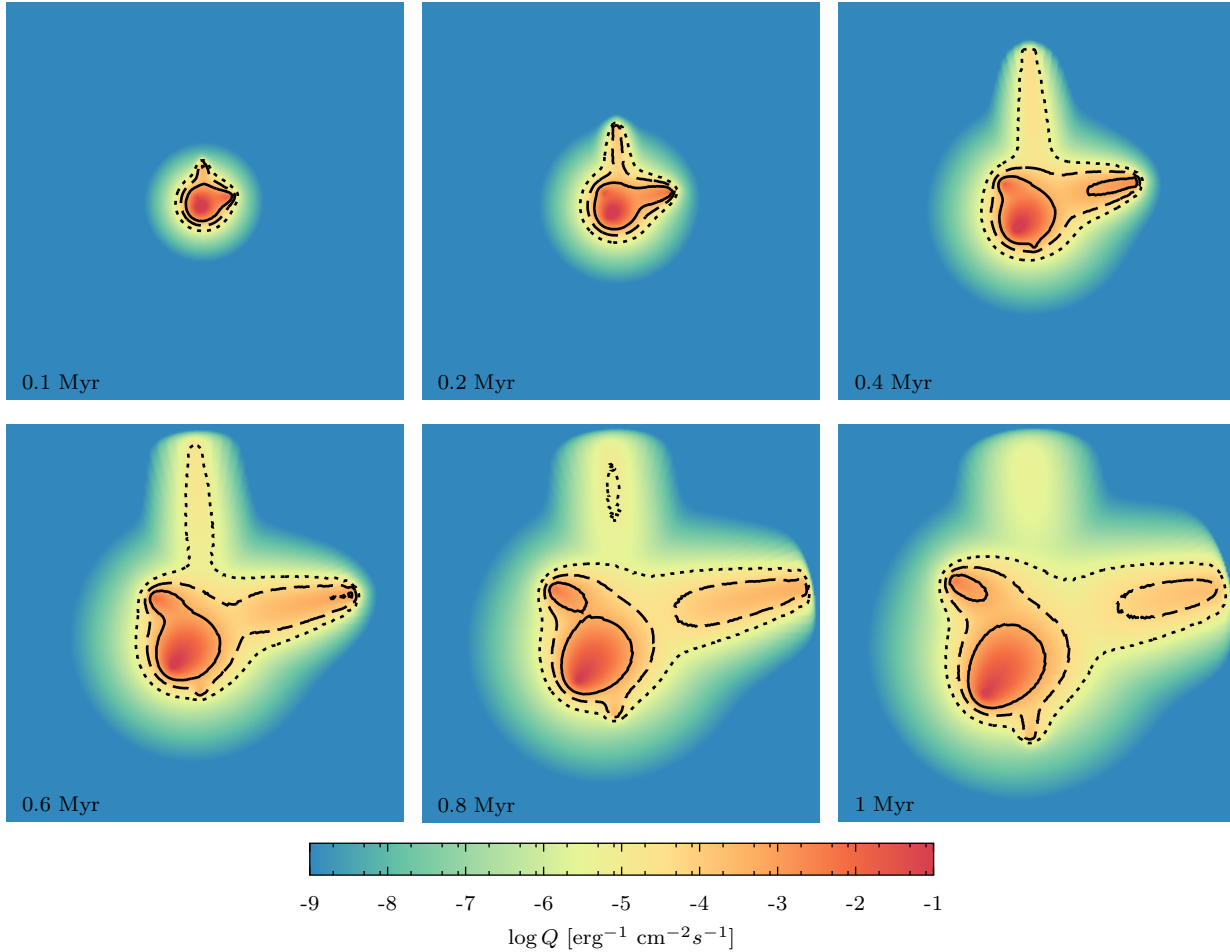
Figure 6. Same as Fig. 5 for slow diffusion ( \chi = 10^{-3} ).
