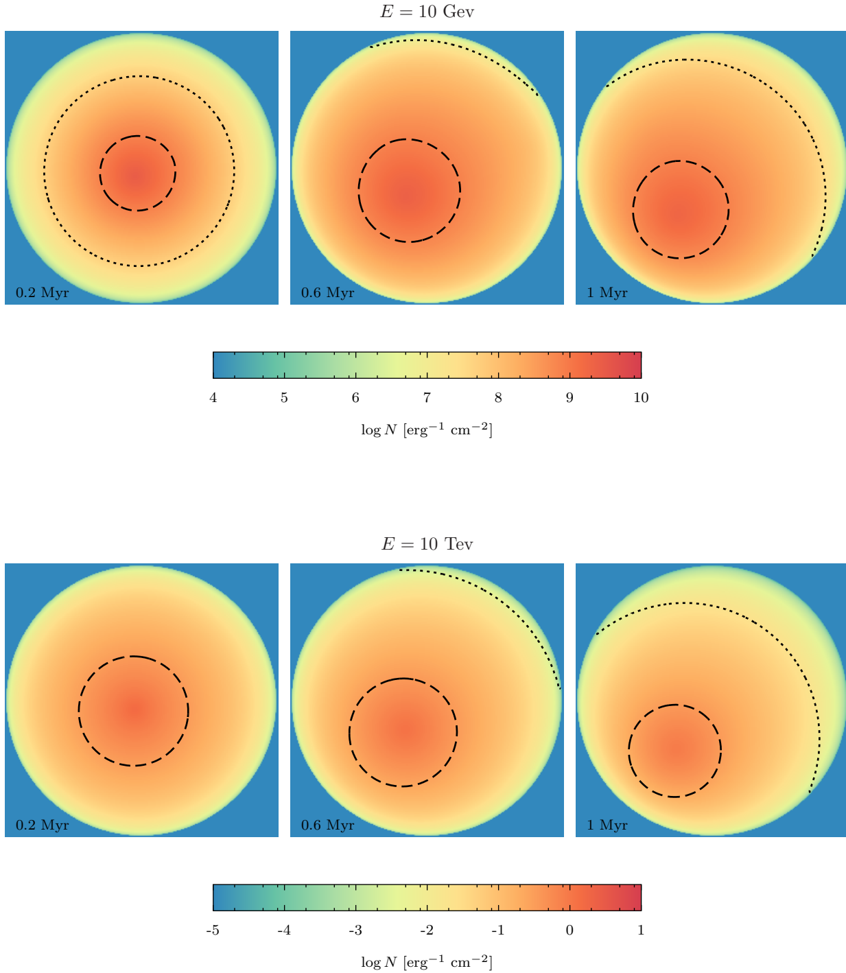
Figure 4. Distribution of e^\pm pairs at fixed energy projected along the line of sight for the case \chi = 10^{-1} . Top: E_e = 10 \text{ GeV} ; bottom: E_e = 10 \text{ TeV} . Time evolves from left to right. The level curves correspond to 0.1 (dotted), and 1 (dashed) times the pairs background distribution.
