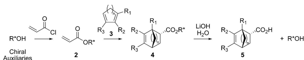
Scheme 2 Chiral auxiliaries derived from levoglucosenone in asymmetric Diels–Alder reactions.
