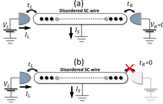
Figure 3. (a) Schematic view of an NSN circuit. (b) Assuming that the coupling to the leads can be controlled in situ experimentally [e.g., using pinch off gates (not shown here)], the system can be effectively disconnected from the right lead and turned effectively into an NS junction.
