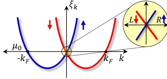
Figure 6. Dispersion relation of a nanowire with Rashba spin-orbit coupling, in the absence of proximity-induced pairing \Delta(x) = 0 , in the absence of Zeeman field V_x = 0 and for \mu_0 = \delta\mu(x) = 0 . Under these conditions, chosen to simplify the theoretical model in Eq. (18), a helical liquid arises near the point k = 0 .
