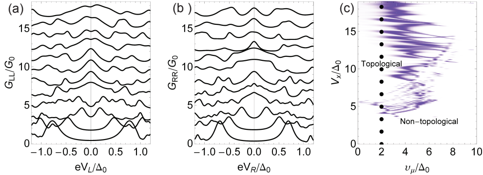
Figure 2. (a) Differential conductance at the left end G_{LL} as a function of the left bias voltage eV_L , for different values of the Zeeman field V_x , and at a temperature T/\Delta_0 = 0.02 , which corresponds to the experimental temperature T_{\text{exp}} \approx 60 mK (see e.g. Ref. [9]). The curves have been shifted vertically for clarity. (b) Idem for the conductance at the right end G_{RR} as a function of the right bias voltage eV_R . In both Figs. 2(a) and 2(b) the zero-bias peaks are smeared by temperature, disorder and quasiparticle broadening arising from the coupling to the normal leads, and they appear at different values of the Zeeman field [see Figs. 4(a) and 4(b) below for more details], complicating the physical interpretation. (c) Color map of the thermal transmission probability \mathcal{T}_{1N} as function of Zeeman field V_x and disorder strength v_\mu . The blue regions correspond to values close to the maximum \mathcal{T}_{1N} = 1 and therefore correspond to the location of the topological quantum phase transition. Each dot corresponds to each one of the curves in Figs. 2(a) and 2(b).
