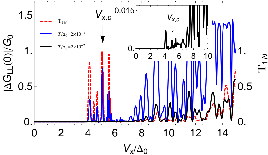
Figure 5. Solid lines represent |\Delta G_{LL}(0)| in Eq. (17) as a function of V_x at T/\Delta_0 = 0.02 (black line) comparable to the experimental temperature T_{\text{exp}} \approx 60 mK, and at T/\Delta_0 = 0.002 (blue line). These curves approximately follow the (thermal) transmission probability \mathcal{T}_{1N} (dashed red line), which shows a maximum \mathcal{T}_{1N} = 1 at V_{x,c}/\Delta_0 \approx 5.2 , corresponding to the TQPT (see arrow). All curves have been calculated with the same configuration of the disorder potential as in Figs. 2 and 4, and correspond to v_\mu/\Delta_0 = 2 [i.e., line of dots in Fig. 2(c)]. Inset: Plot of |\Delta G_{LL}(0)| at T/\Delta_0 = 0.02 in a smaller scale showing that, although weaker, the signal persists and is still experimentally measurable.
