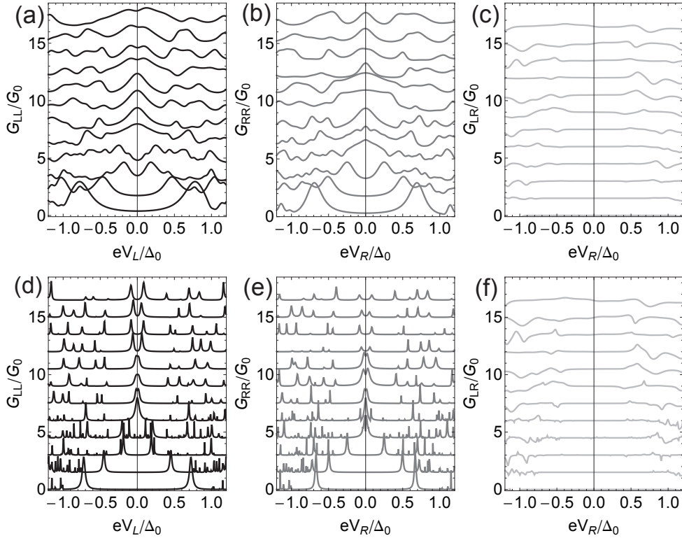
Figure 4. (a) Differential conductances G_{LL} vs V_L , (b) G_{RR} vs V_R and (c) G_{LR} vs V_R . All the curves in the top [i.e., (a), (b) and (c)] have been computed at a temperature T/\Delta_0 = 0.02 (corresponding to the experimental temperature T_{\text{exp}} \approx 30 mK) and for effective couplings to the leads \gamma_L = 0.85 t and \gamma_R = 0.95 t . Figs. 4(a) and (b) correspond to Figs. 2(a) and (b) and exemplify the potential difficulties in detecting the TQPT in a disordered Majorana wire, with non-topological ZBPs appears at finite Zeeman field. In the bottom plots [i.e., (d), (e) and (f)] we show the same quantities computed at much lower a temperature T/\Delta_0 = 2 \times 10^{-4} (below experimental capabilities) and for effective couplings to the leads \gamma_L = \gamma_R = 0.1 t . In these conditions, the widths of the conductance peaks decrease dramatically, revealing the splitting of the ZBPs due to disorder.
