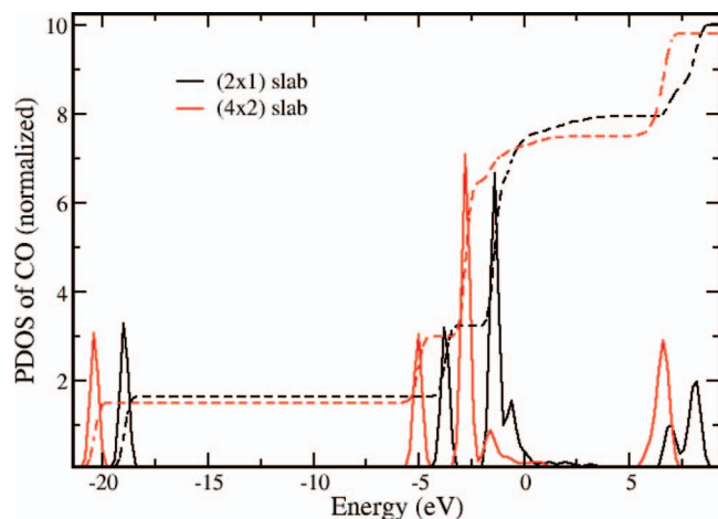
FIG. 3. Density of states projected on the atomic orbitals of the CO molecule adsorbed at the bridging-oxygen site, in the (4×2) and (2×1) model slabs of the rutile (110) surface. The dashed lines show the integration of the projected density of states. The smaller charge integrated for the (4×2)-cell reflects a higher delocalization of the electronic density around the defect, with respect to the (2×1)-cell.
