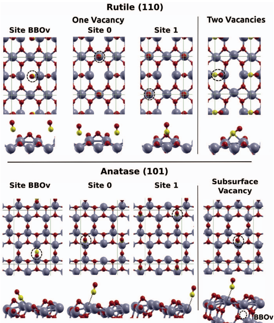
FIG. 2. Top and side views of the optimized, reduced TiO 2 surface models, including the adsorbed CO on the different sites examined. Ti, O, and C atoms are depicted in blue, red, and yellow, respectively. The dashed circles mark the position of the CO molecule (top views) and of the subsurface oxygen vacancy (side view). Ov stands for oxygen vacancy.
